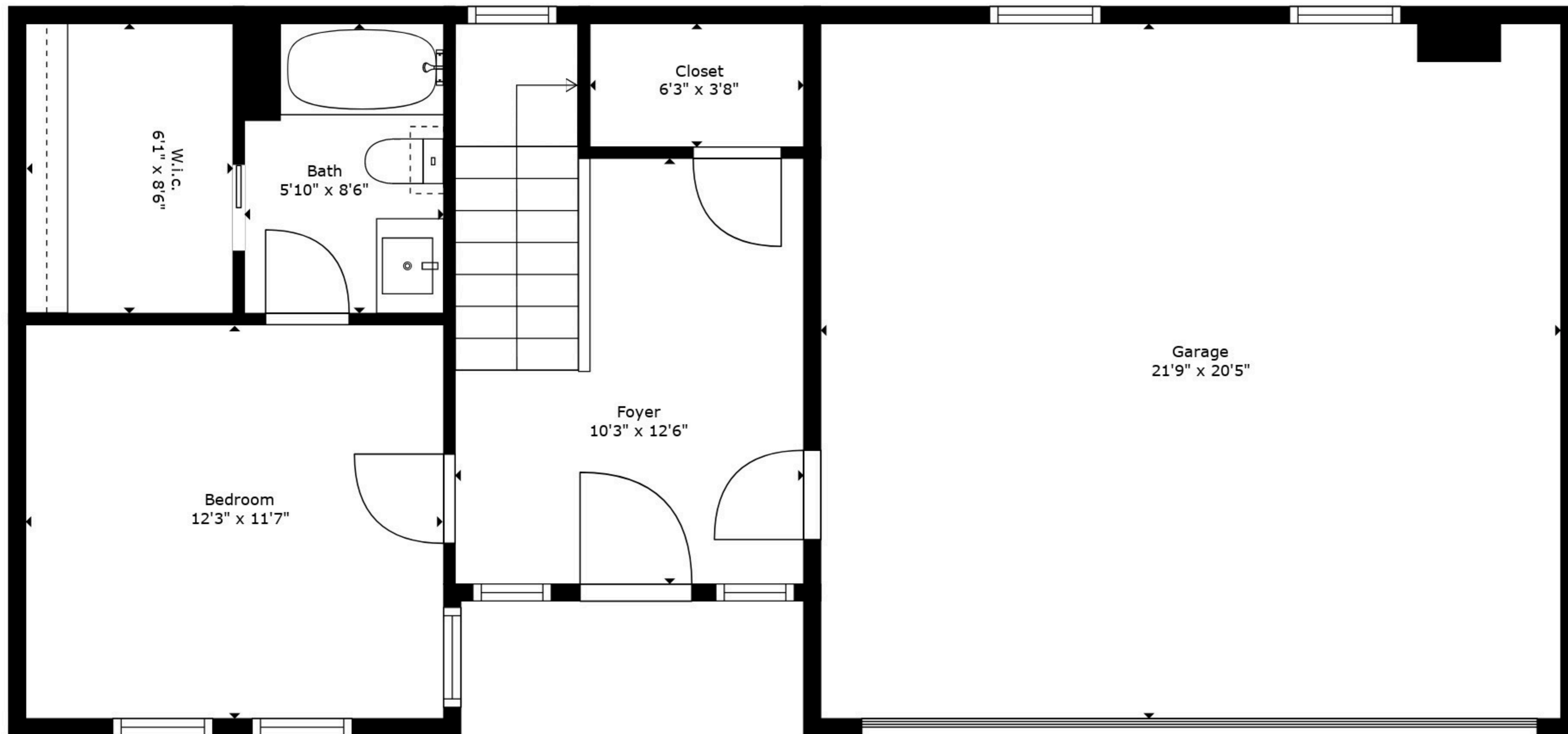
Floor 1
