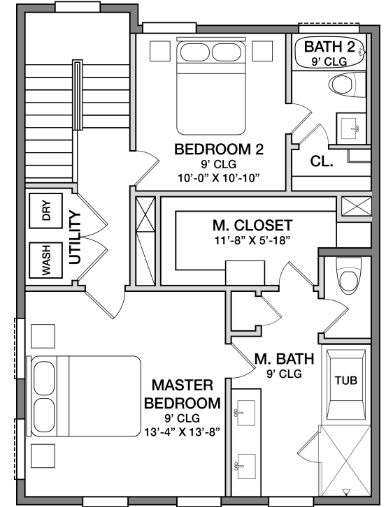
3RD FLOOR
