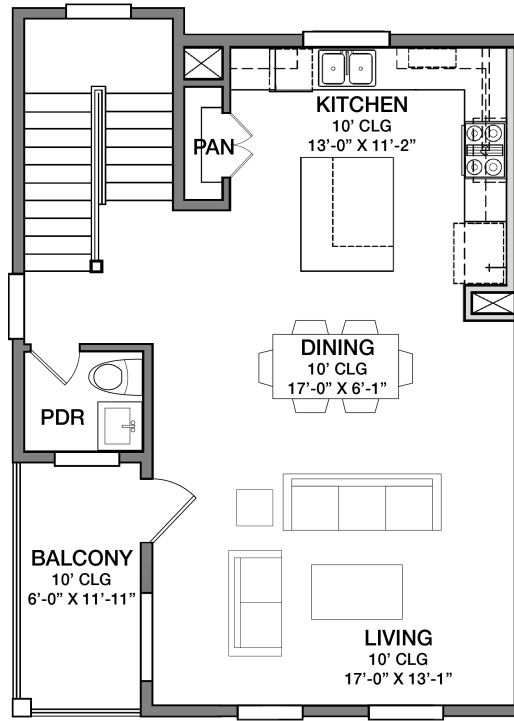
2ND FLOOR
