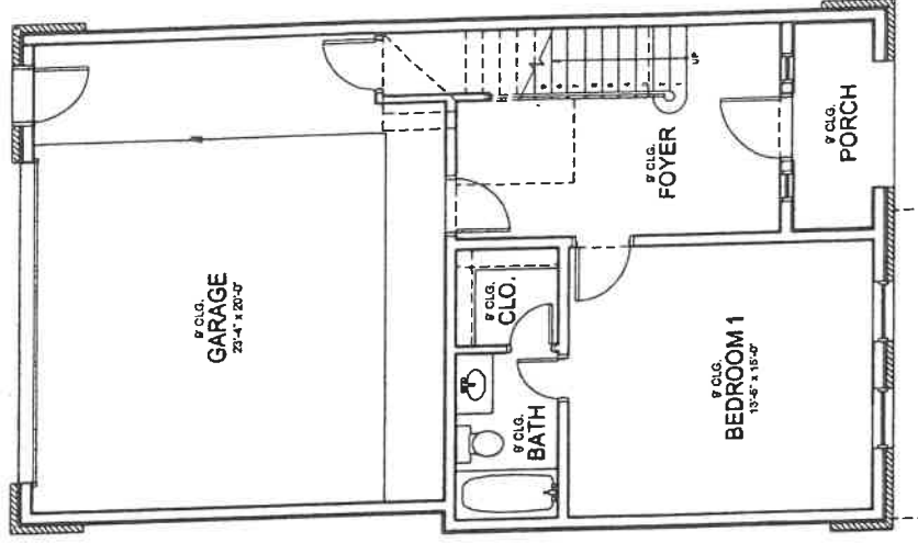
FIRST FLOOR PLAN Scale: 3/16" = 1'-0"
