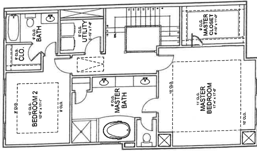
THIRD FLOOR PLAN Scale: 3/16" = 1'-0"
