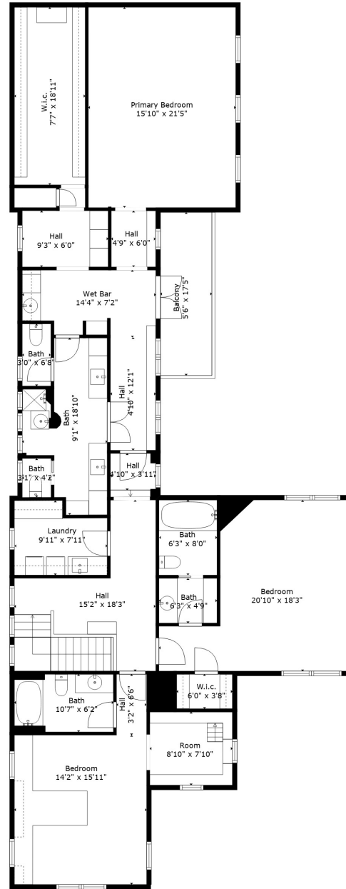
Floor 2
