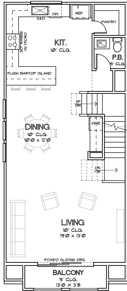
SECOND FLOOR PLAN PLAN 2104
