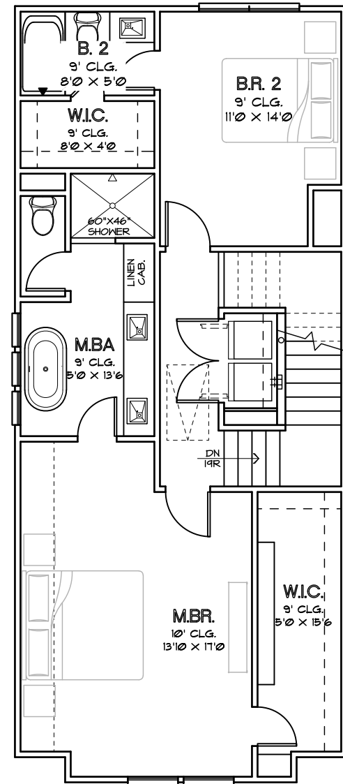
THIRD FLOOR PLAN PLAN 2104
