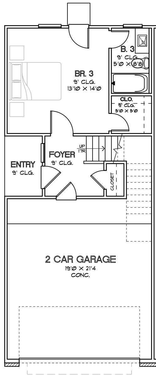
FIRST FLOOR PLAN PLAN 2104
