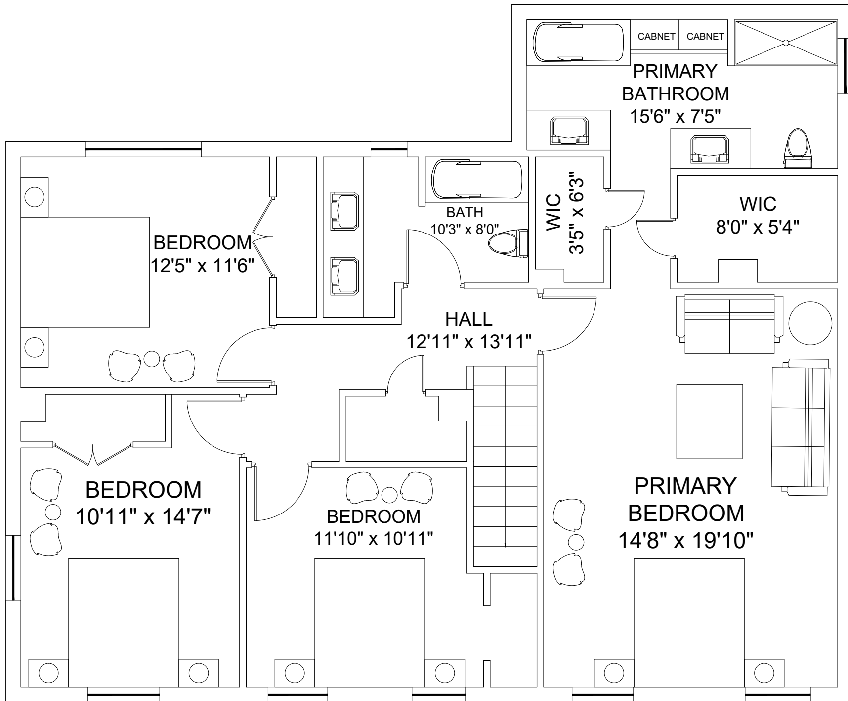
SECOND FLOOR
