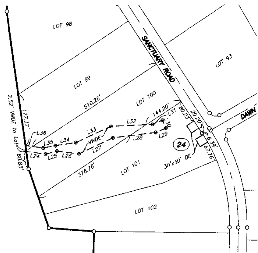
DETAIL VIEW 'F' (See Sheet 5)
