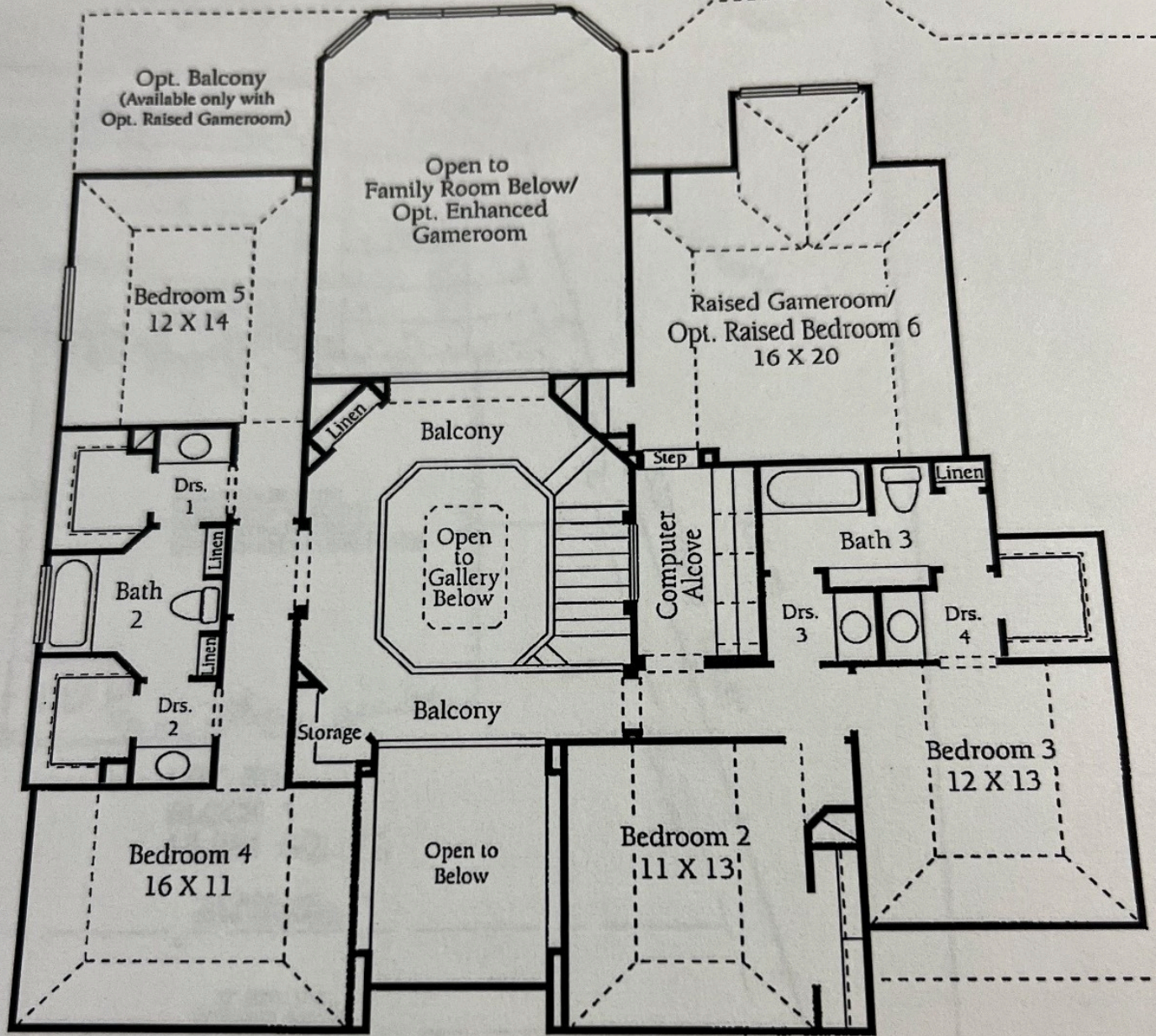
SECOND FLOOR
