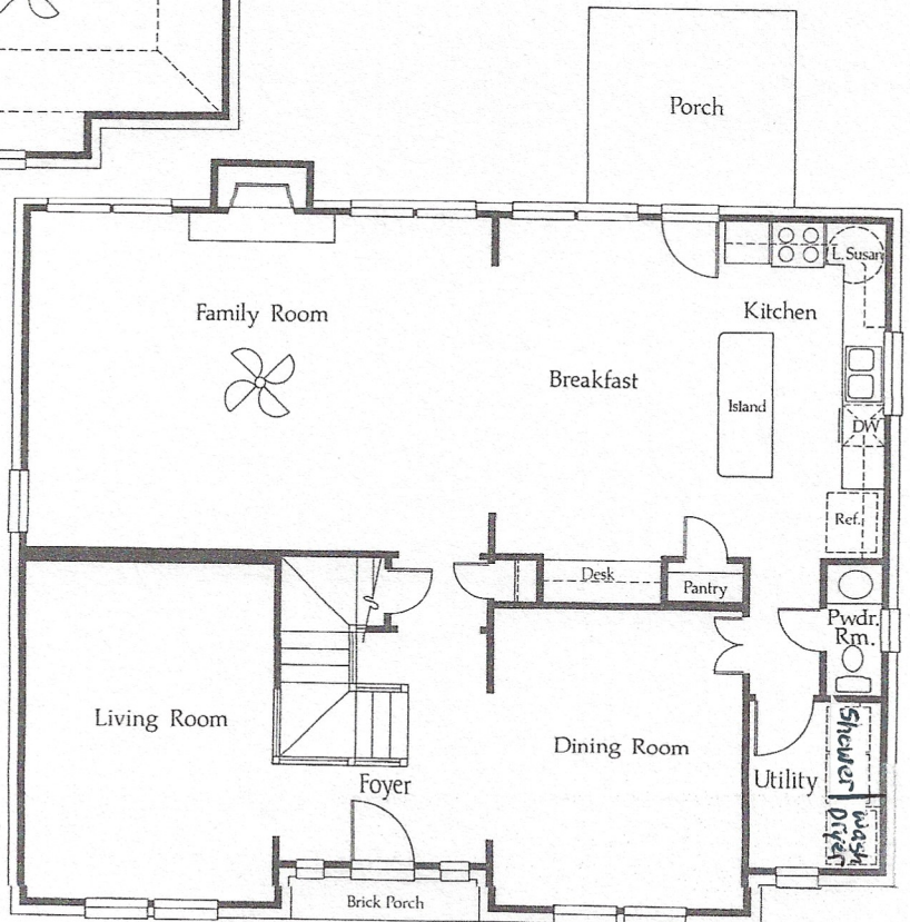
FIRST FLOOR
