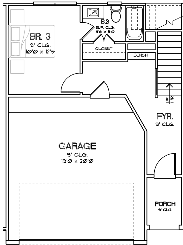
FIRST FLOOR PLAN PLAN 1902
