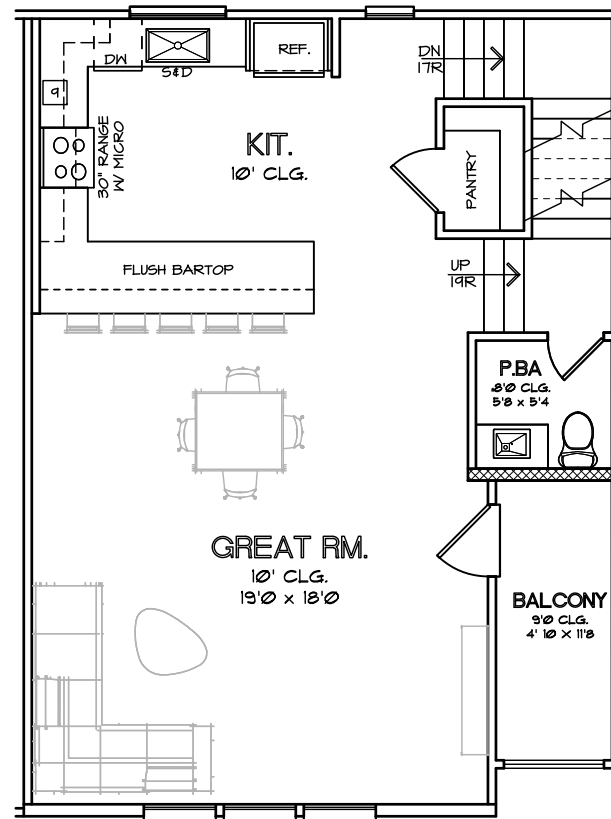
SECOND FLOOR PLAN PLAN 1902
