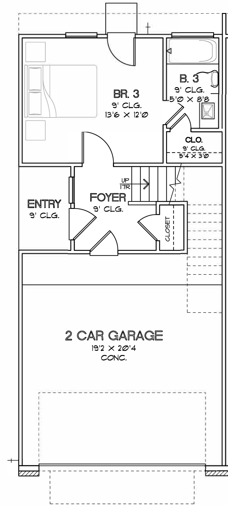
FIRST FLOOR PLAN PLAN 2083
