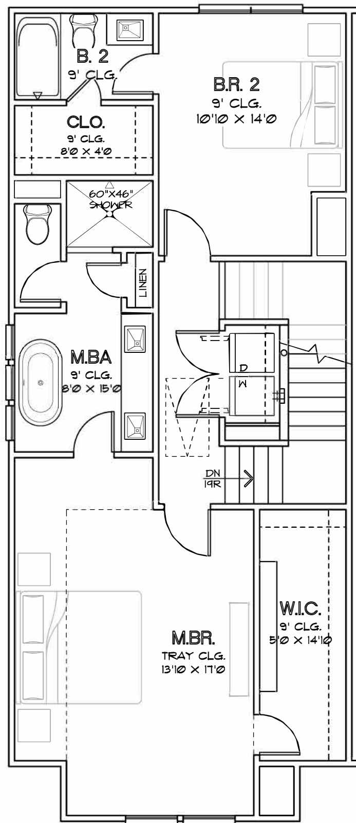
THIRD FLOOR PLAN PLAN 2083
