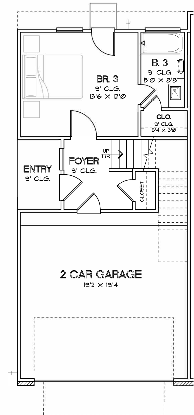
FIRST FLOOR PLAN PLAN 2053
