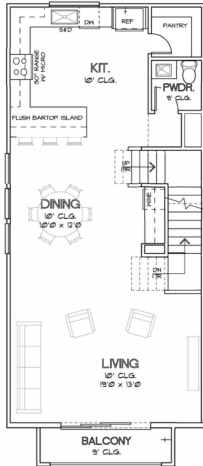
SECOND FLOOR PLAN PLAN 2053
