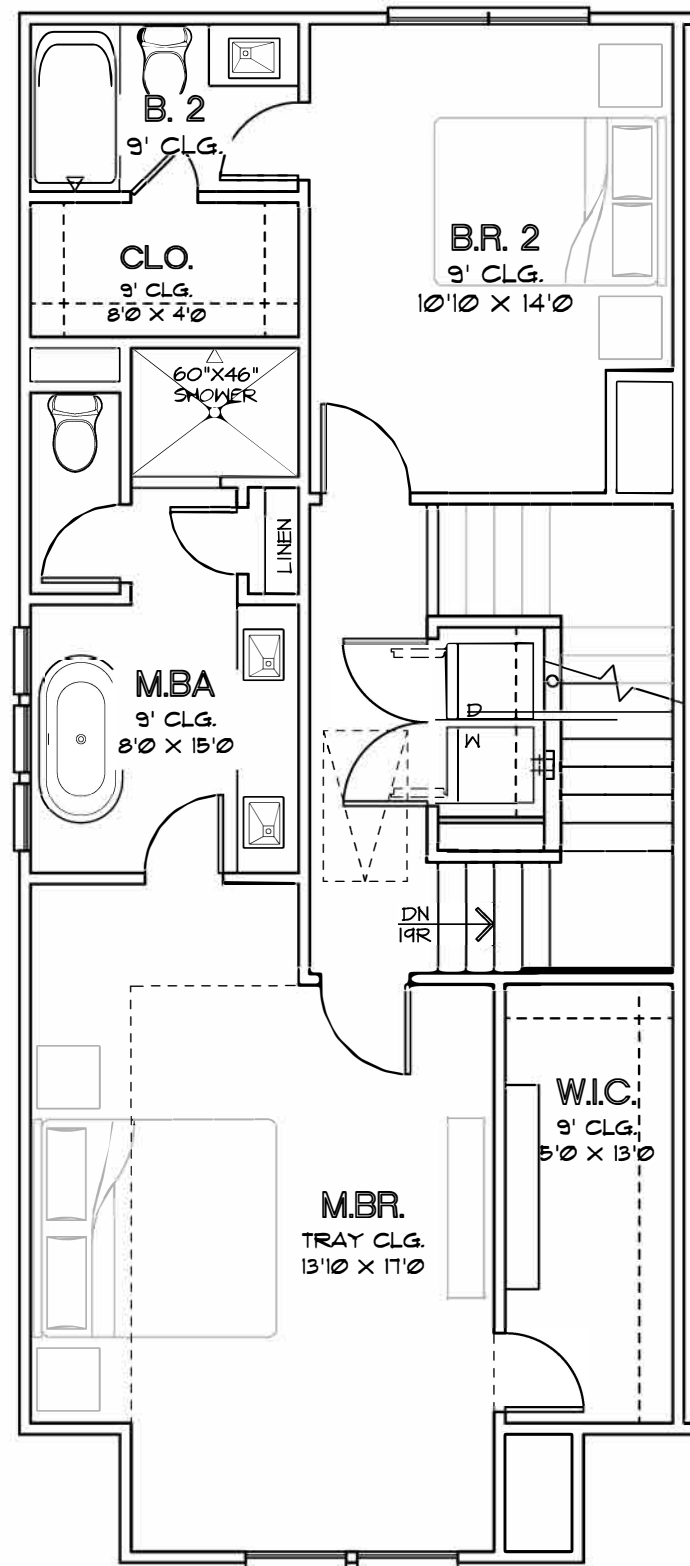
THIRD FLOOR PLAN PLAN 2053
