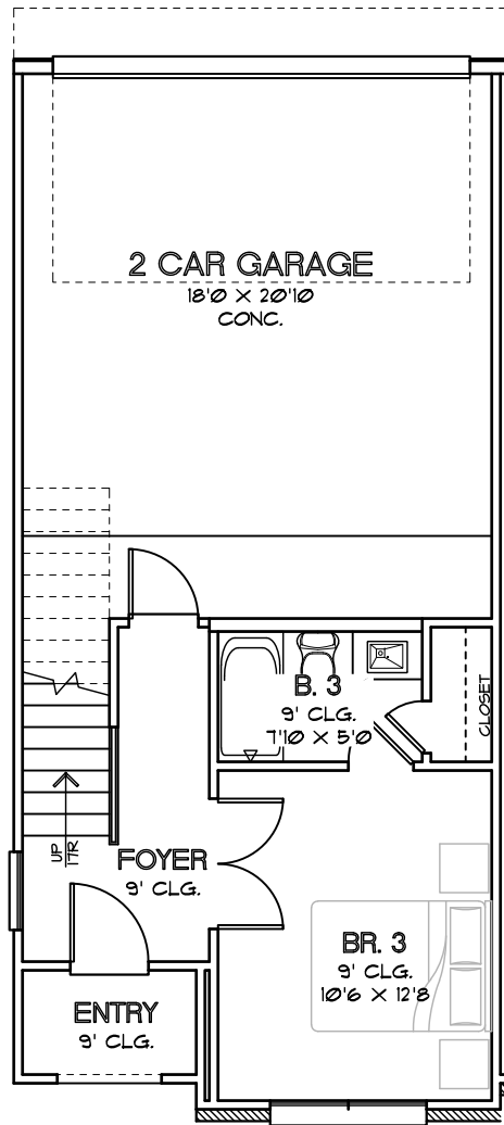
FIRST FLOOR PLAN PLAN 1786
