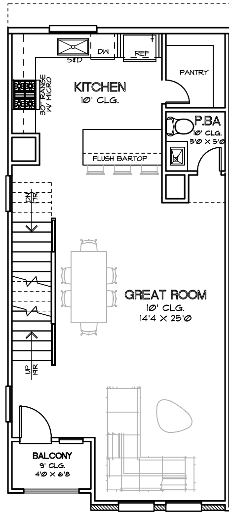
SECOND FLOOR PLAN PLAN 1786
