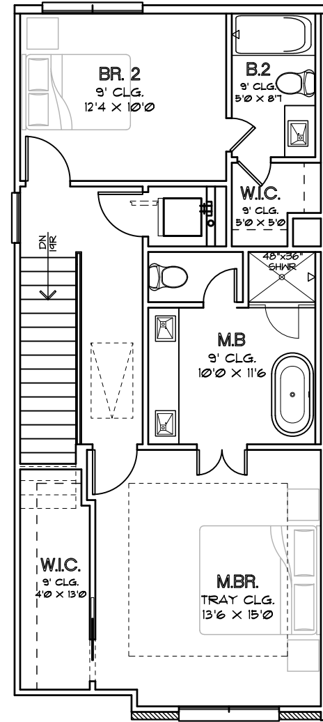
THIRD FLOOR PLAN PLAN 1786
