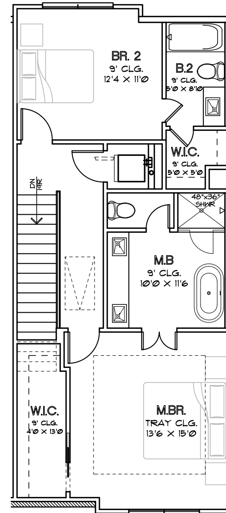
THIRD FLOOR PLAN PLAN 1871
