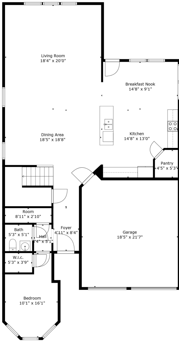
Floor 1
