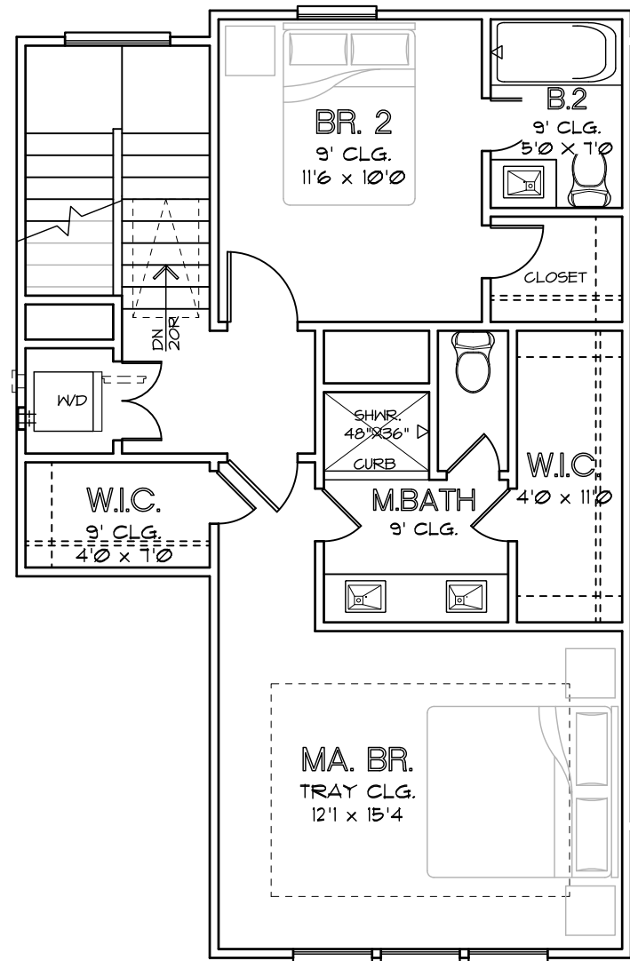
THIRD FLOOR PLAN PLAN 1457 L
