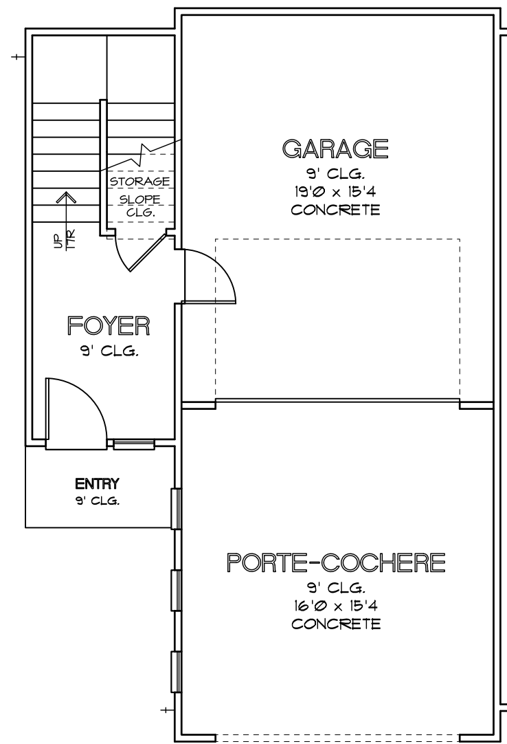
FIRST FLOOR PLAN PLAN 1457 L
