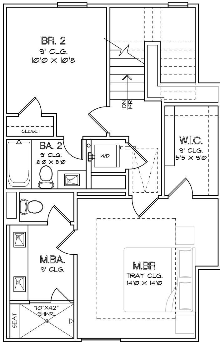
THIRD FLOOR PLAN PLAN 1700 R
