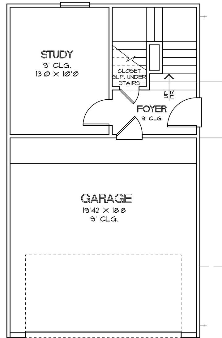
FIRST FLOOR PLAN PLAN 1700 R
