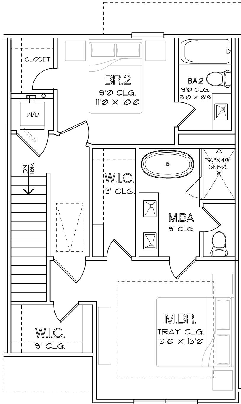
THIRD FLOOR PLAN PLAN 1650
