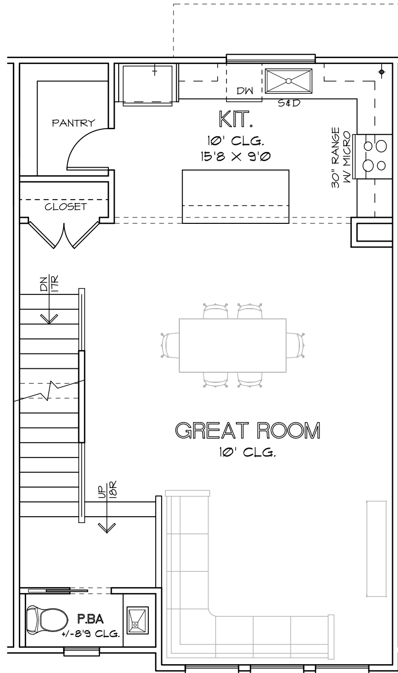
SECOND FLOOR PLAN PLAN 1650
