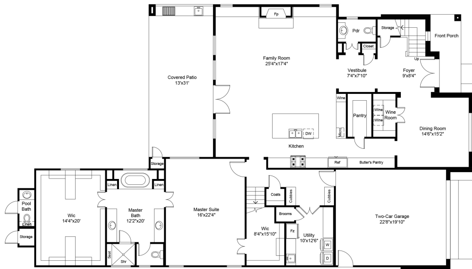
FIRST FLOOR PLAN ON SITE PLAN
