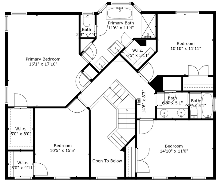
Floor 2
