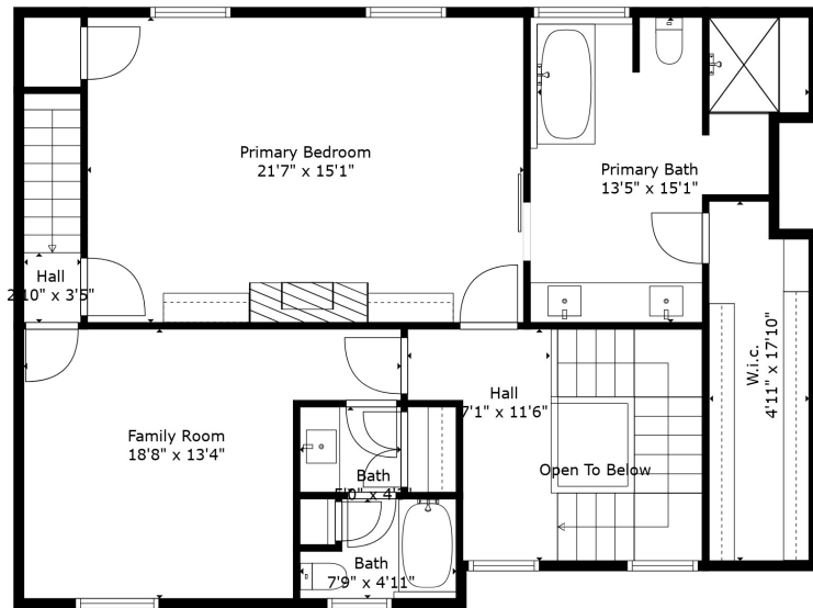
Floor 3
