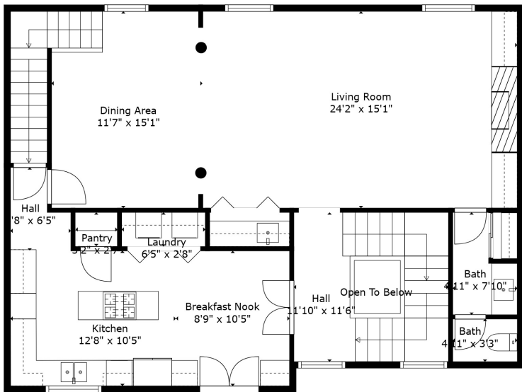
Floor 2
