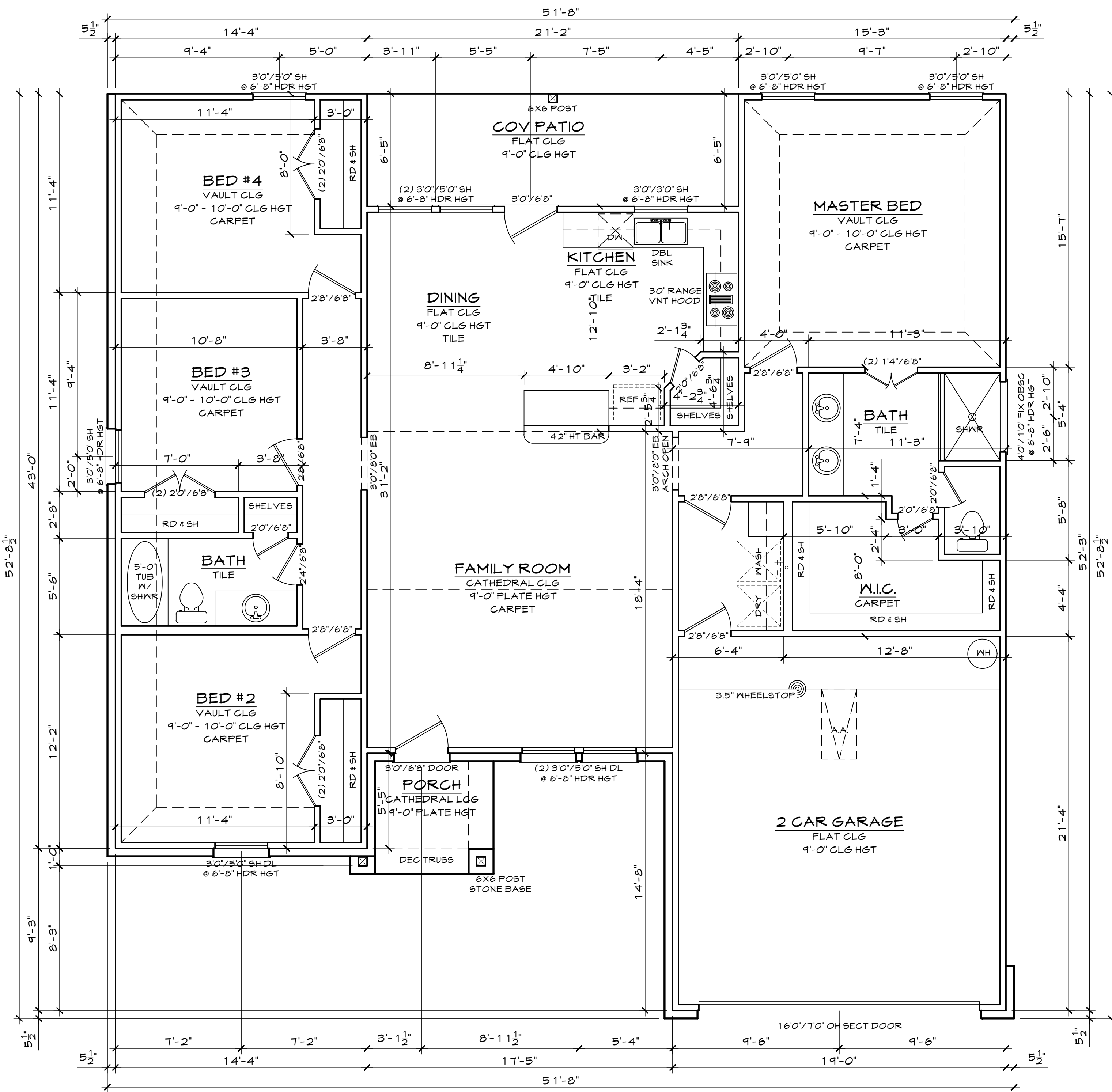
1 FLOOR PLAN SCALE: 1/4" = 1'
