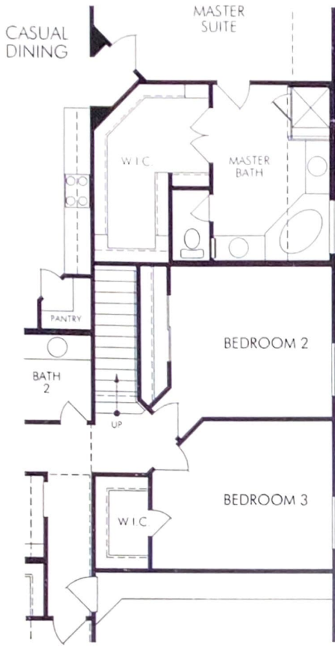
OPT. STAIRS WITH SECOND FLOOR BONUS ROOM UPSTAIRS
