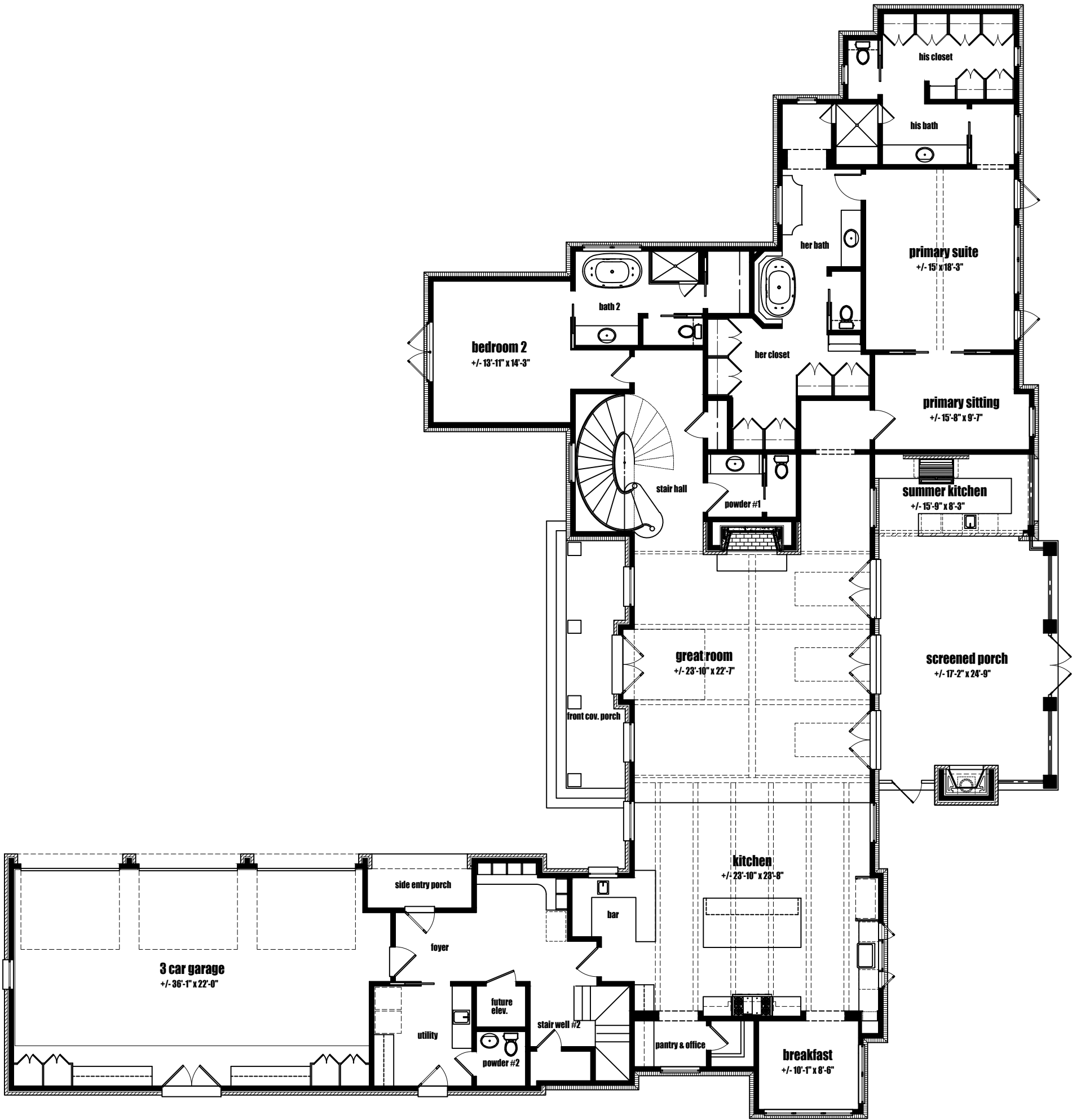
first floor plan scale: no scale
