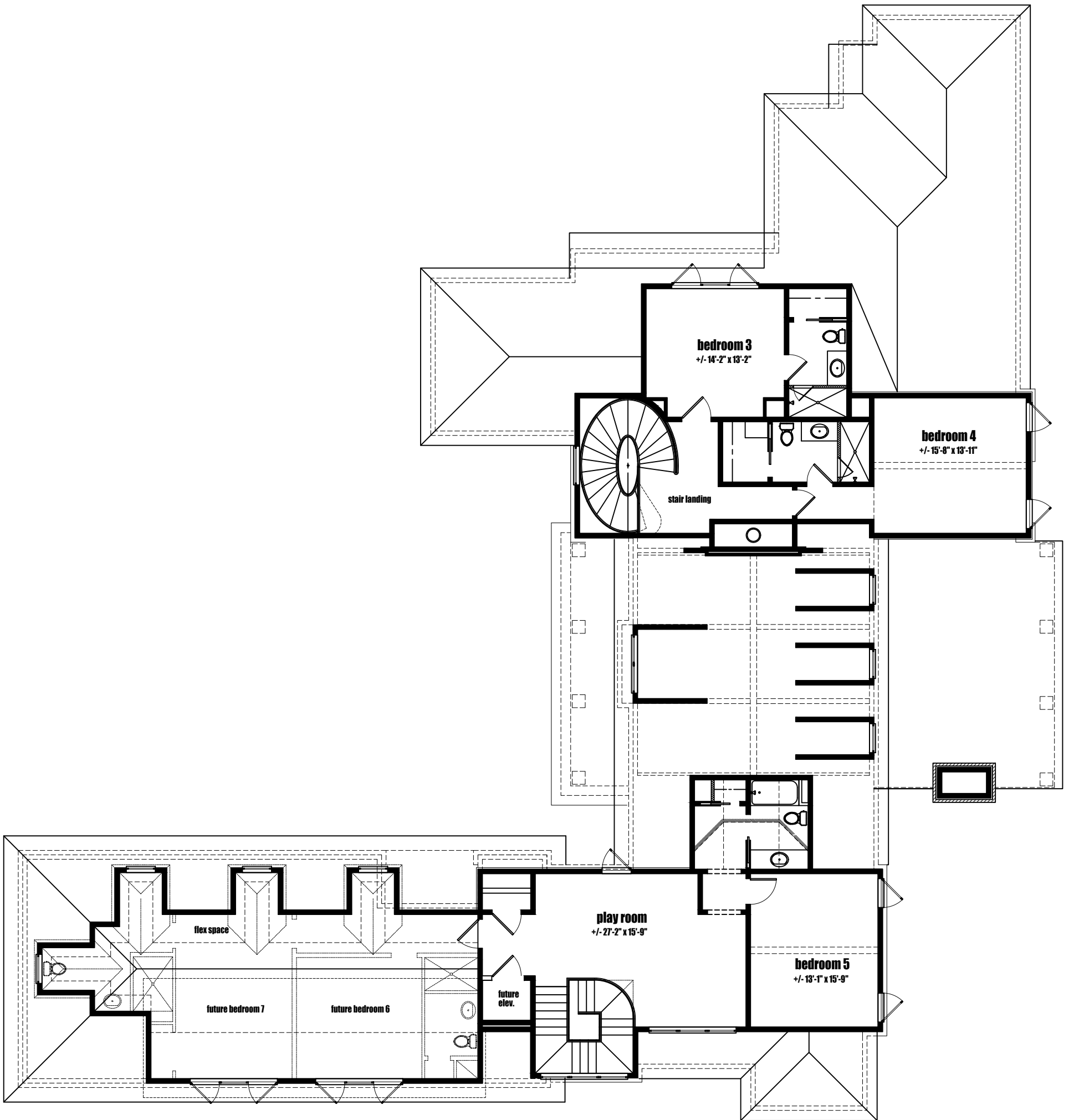
second floor plan scale: no scale
