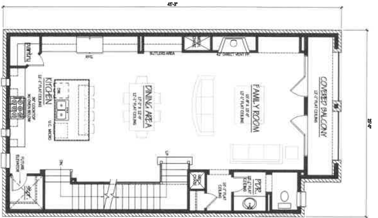
SECOND FLR. SCALE 1/8"=1'-0"
