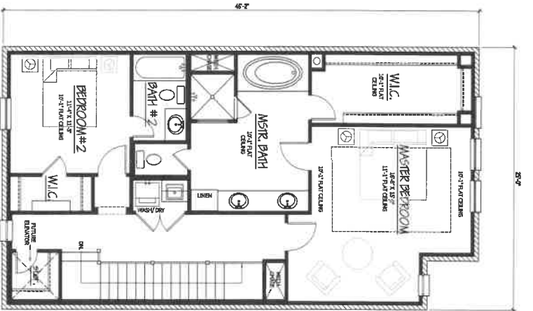
THIRD FLR. SCALE 1/8"=1'-0"
