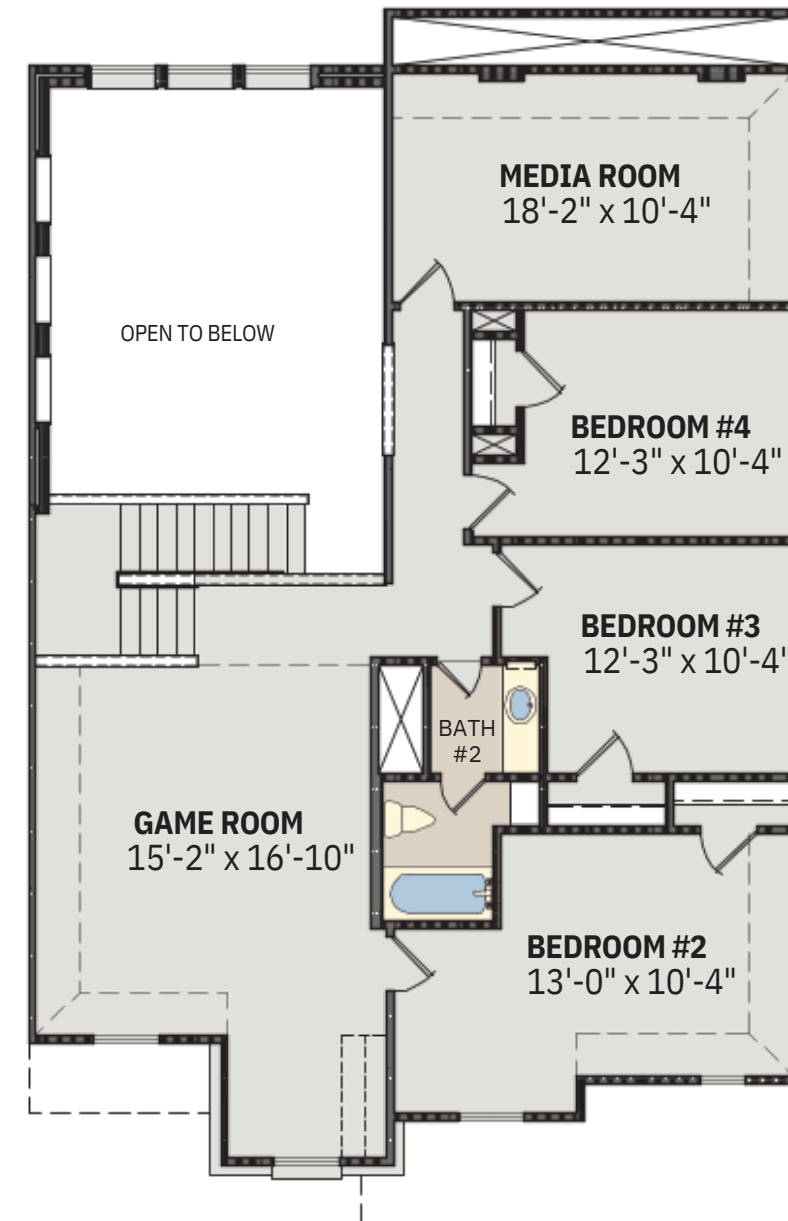
2nd Floor
