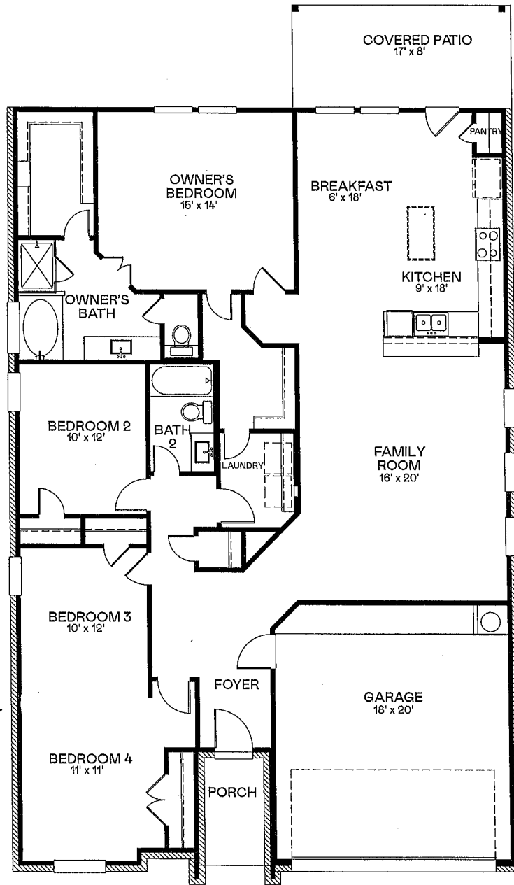
1st floor
