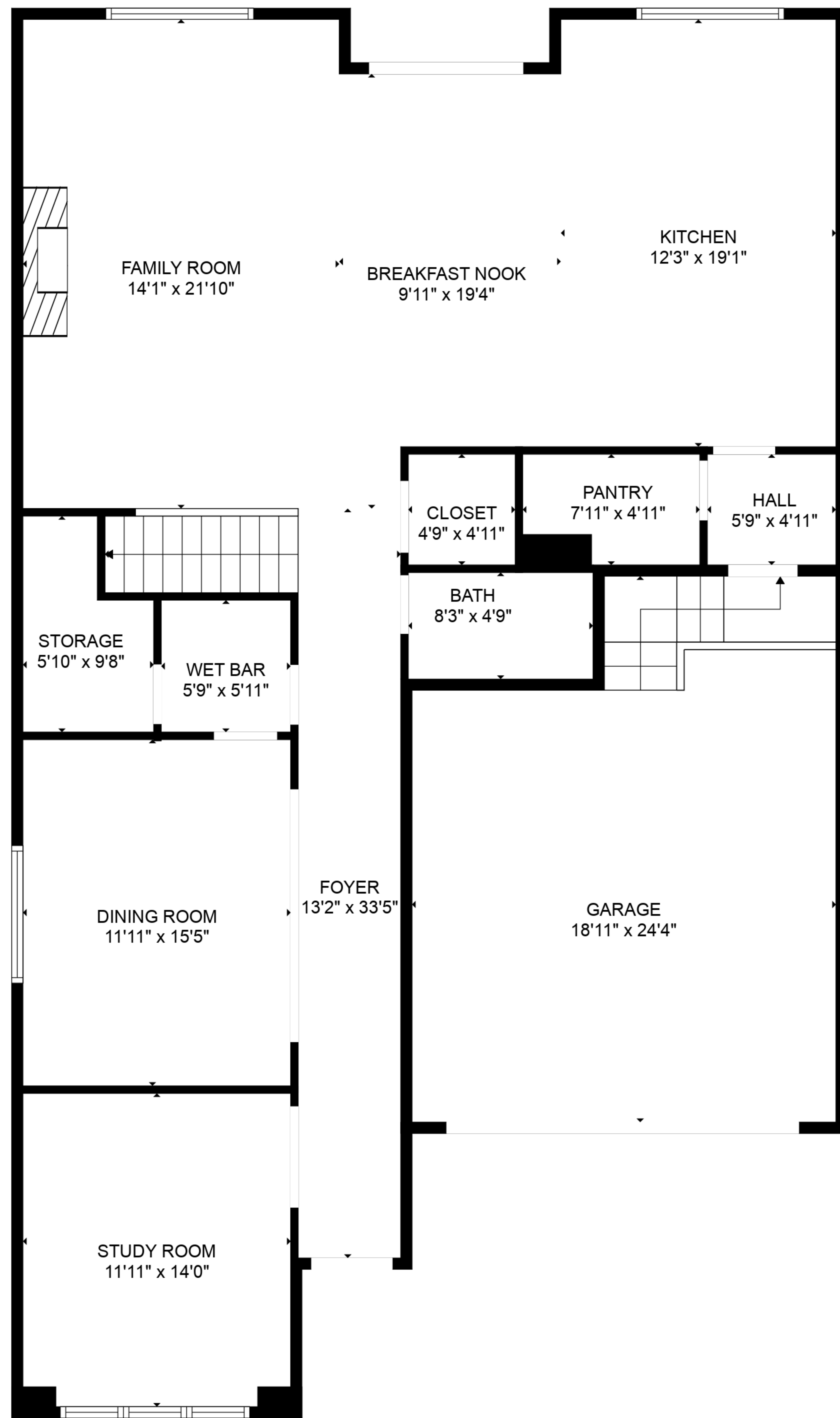
FLOOR 1
