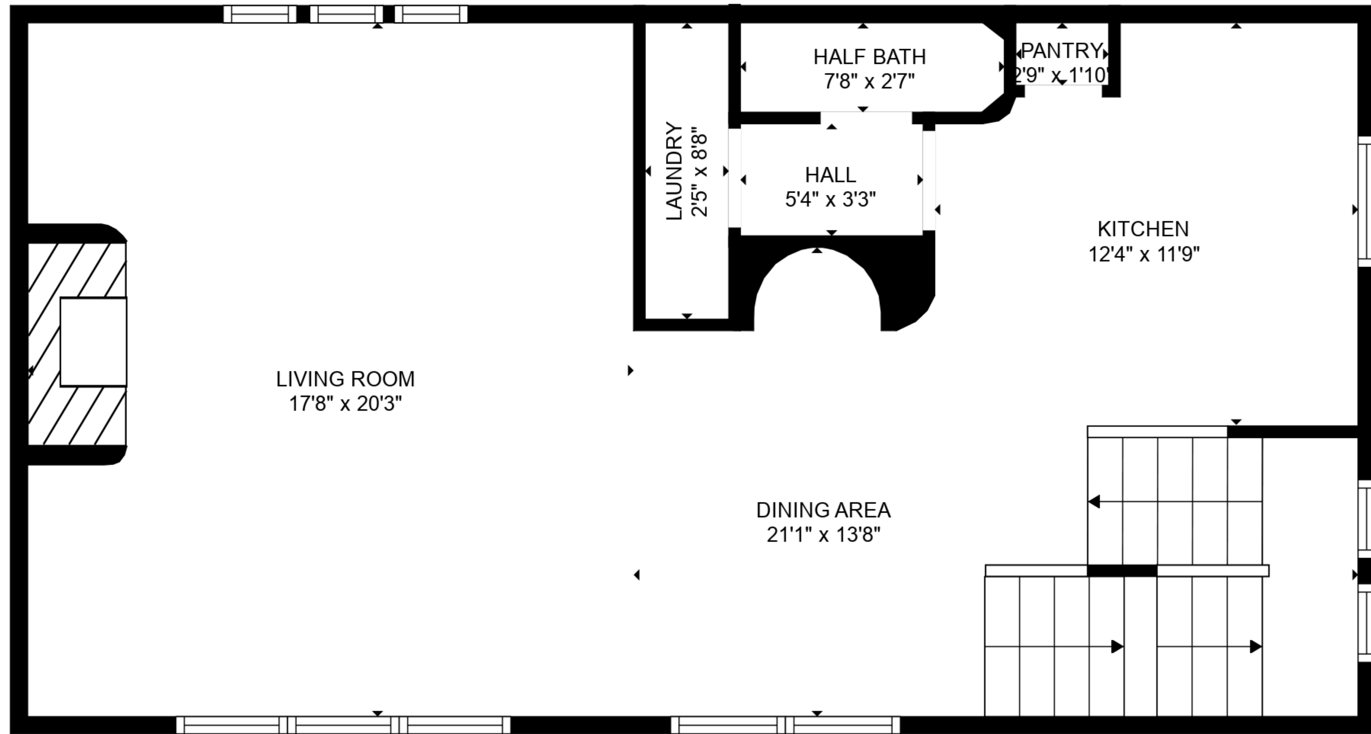
FLOOR 2
