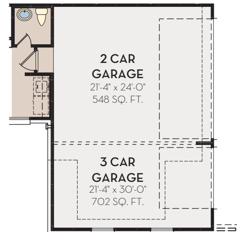
OPT. 2 AND 3 CAR SIDE LOAD GARAGE
