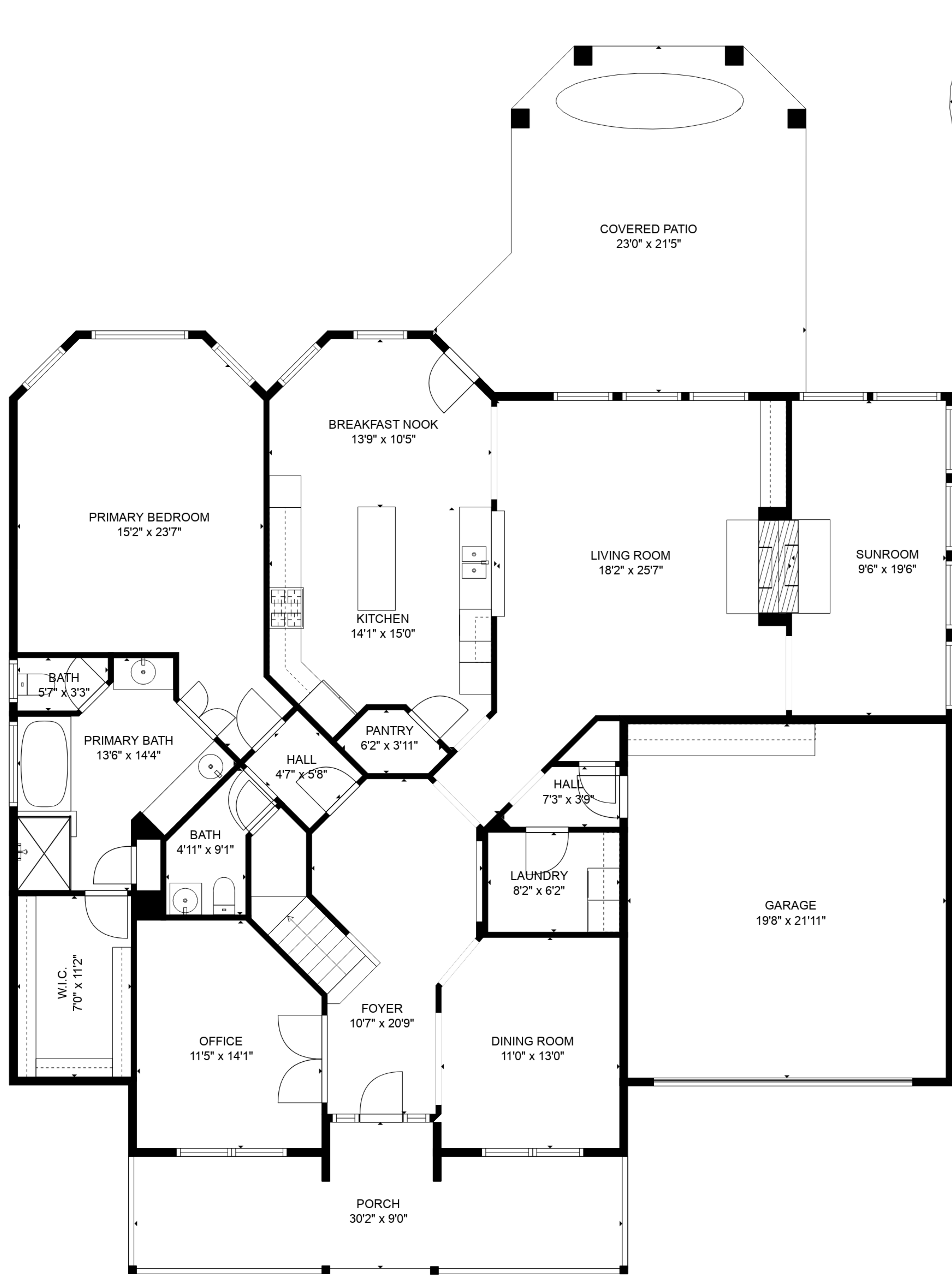
FLOOR 1
