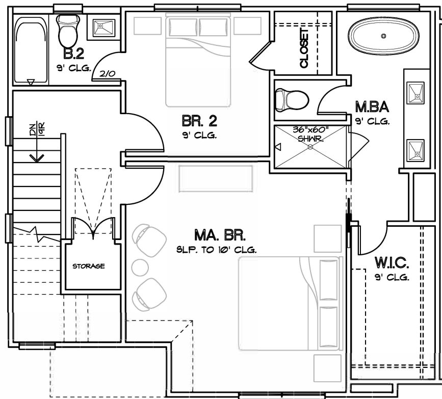
THIRD FLOOR PLAN PLAN 1804
