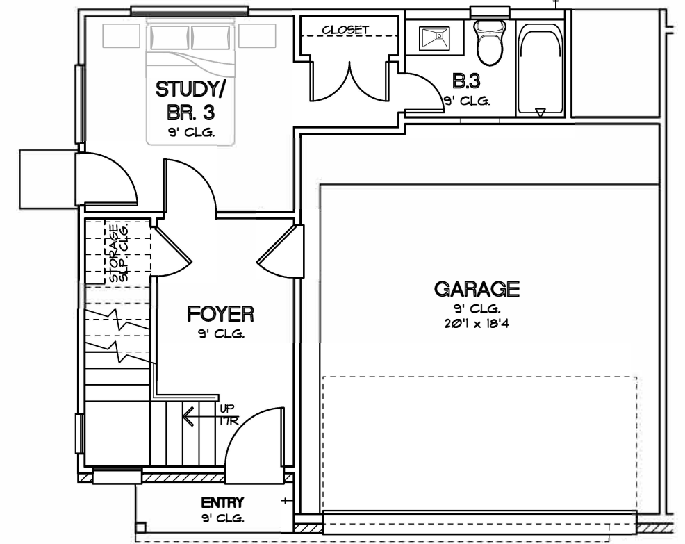
FIRST FLOOR PLAN PLAN 1804
