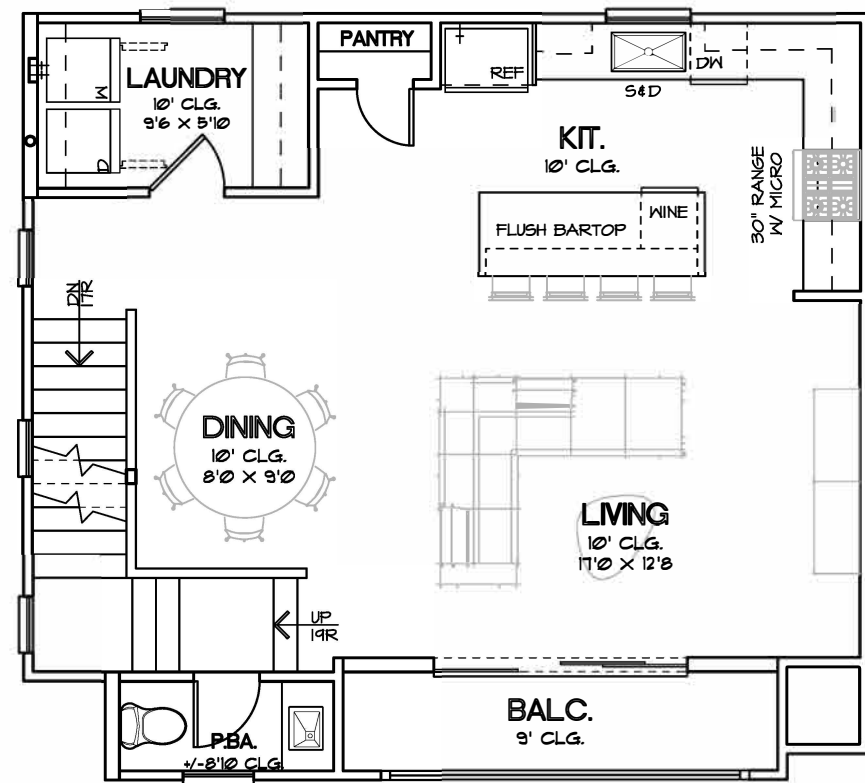
SECOND FLOOR PLAN PLAN 1804
