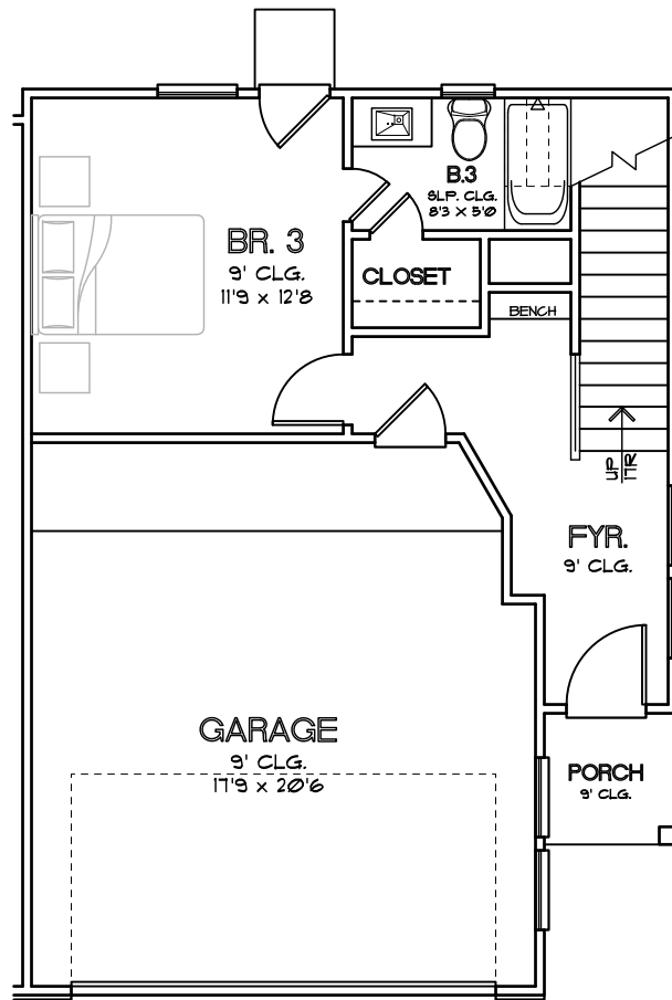
FIRST FLOOR PLAN PLAN 1932
