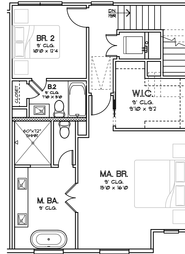
THIRD FLOOR PLAN PLAN 1932
