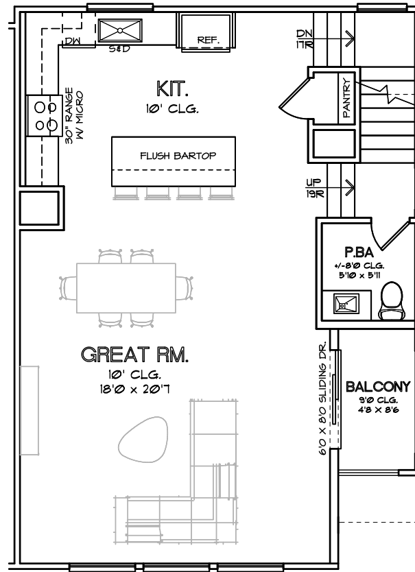
SECOND FLOOR PLAN PLAN 1932
