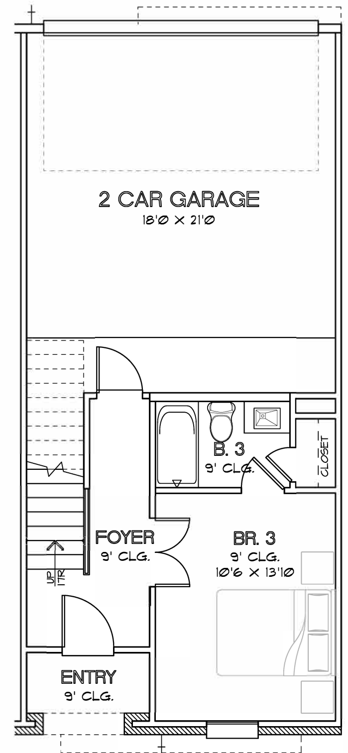
FIRST FLOOR PLAN PLAN 1824
