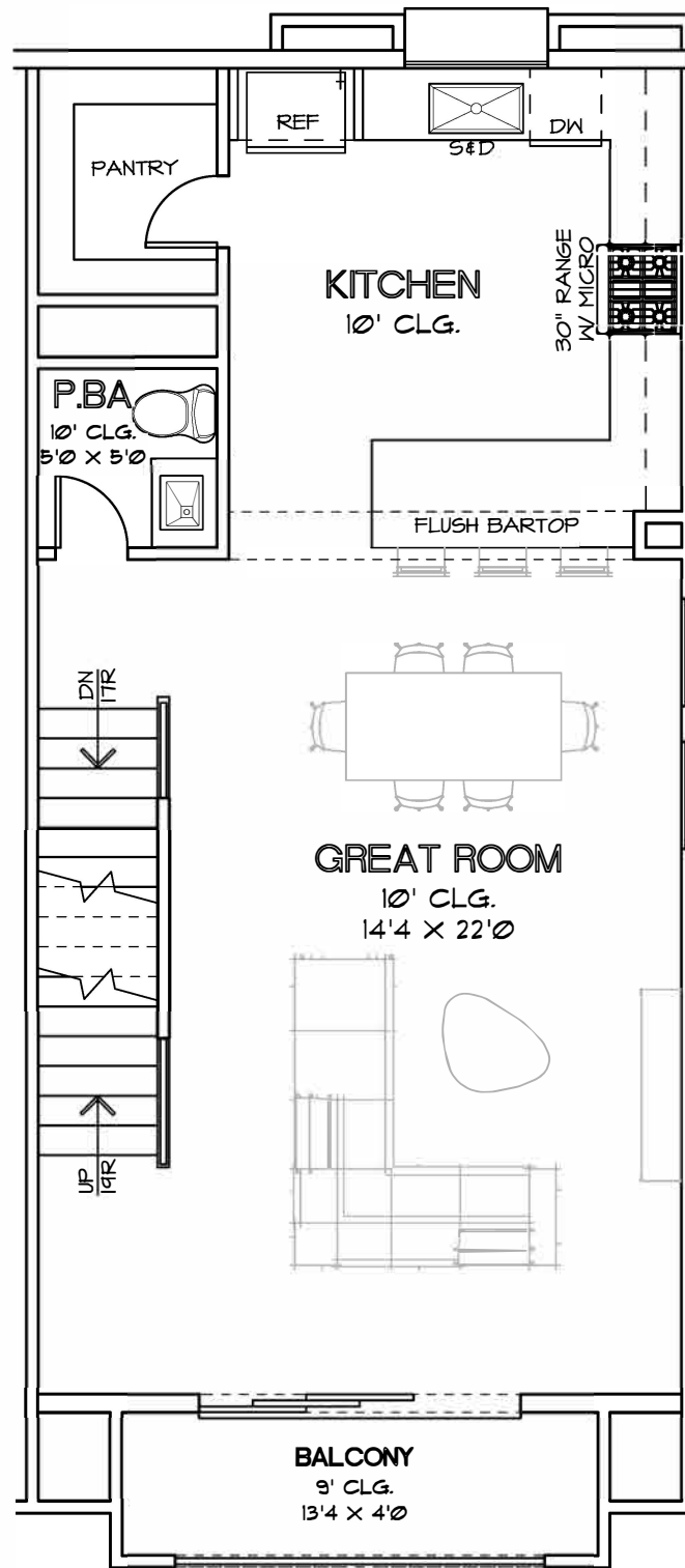
SECOND FLOOR PLAN PLAN 1824
