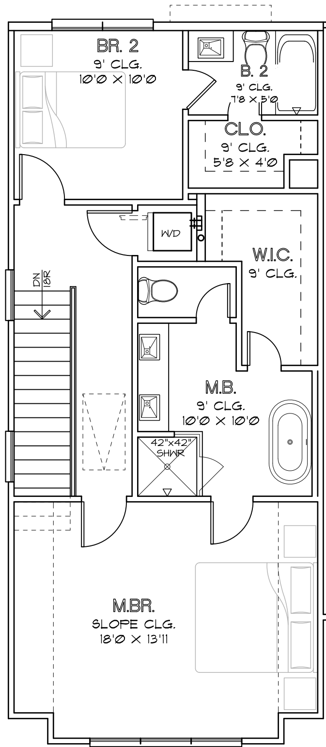
THIRD FLOOR PLAN PLAN 1841 L
