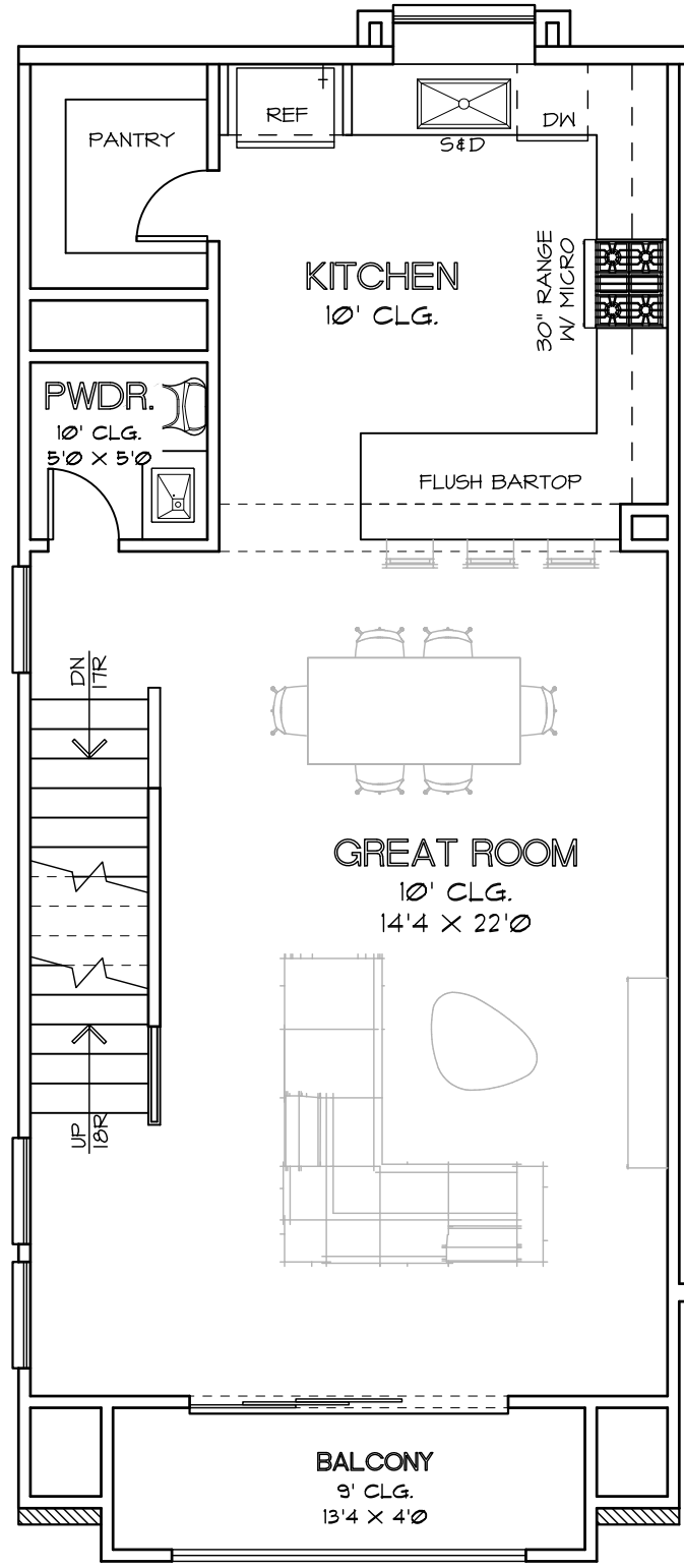
SECOND FLOOR PLAN PLAN 1841 L
