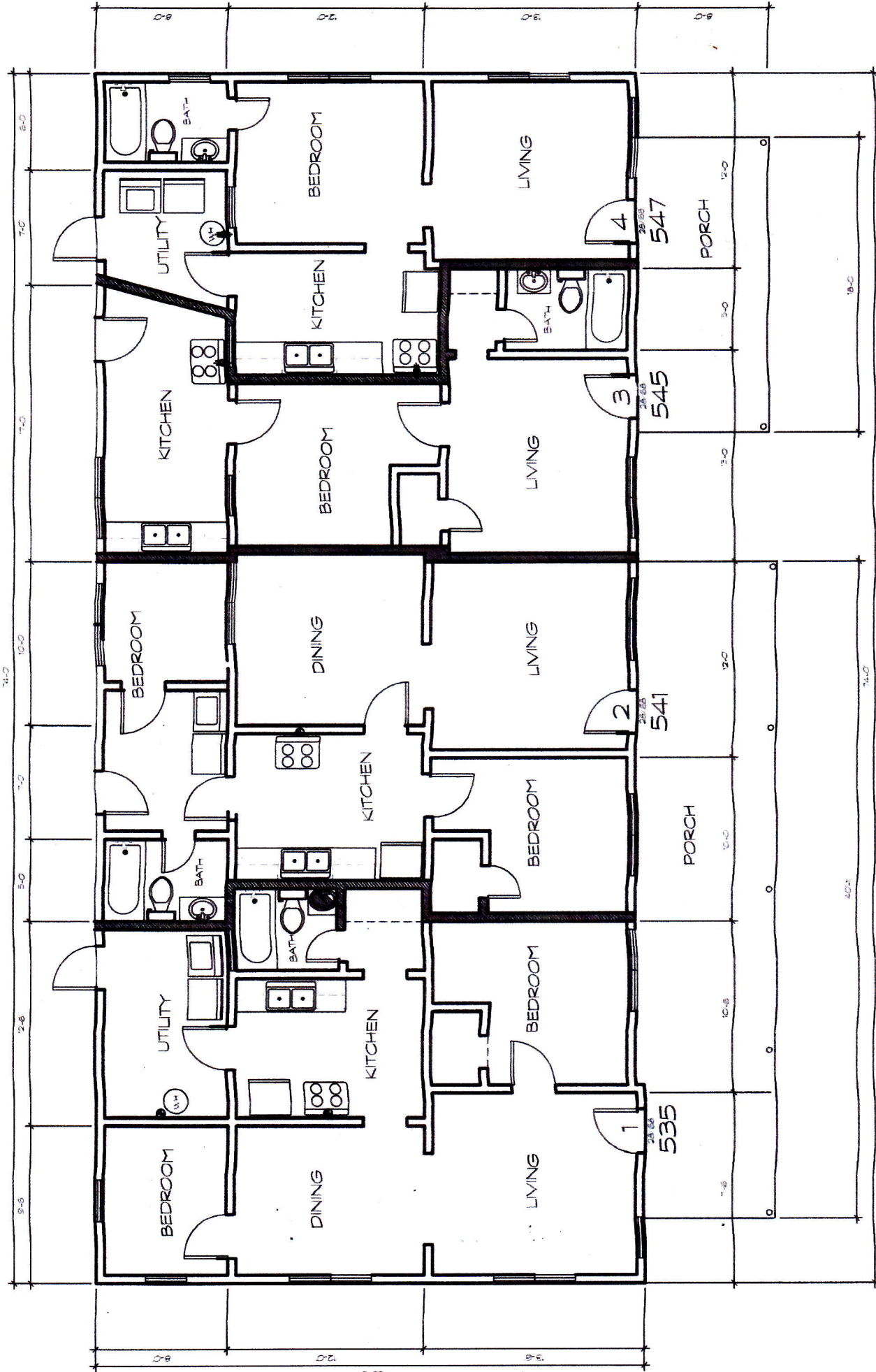
FLOOR PLAN
