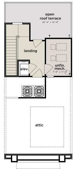
ROOF / TERRACE
