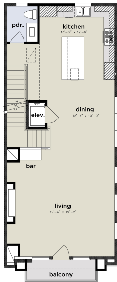
SECOND FLOOR
