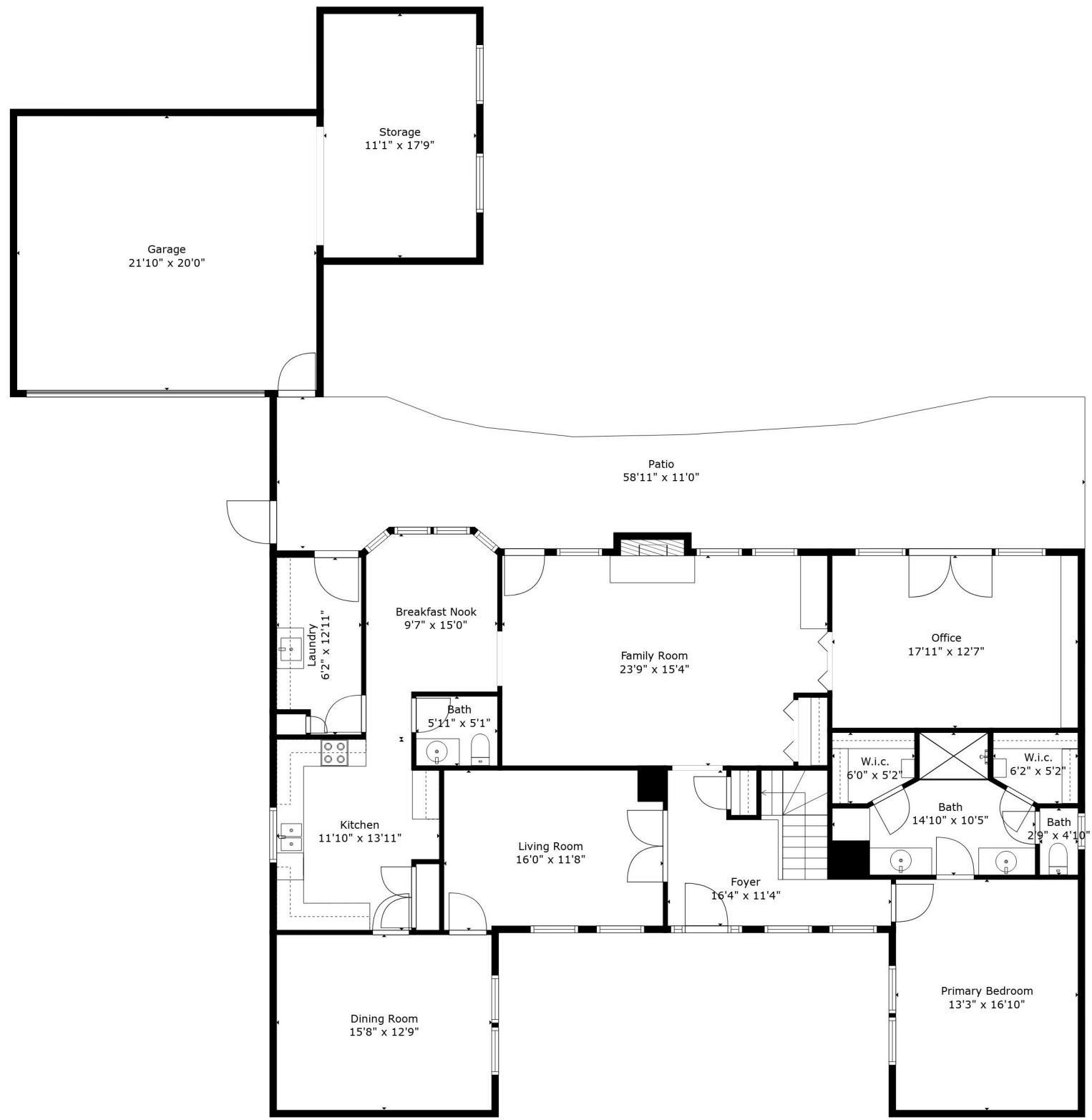
Floor 1
