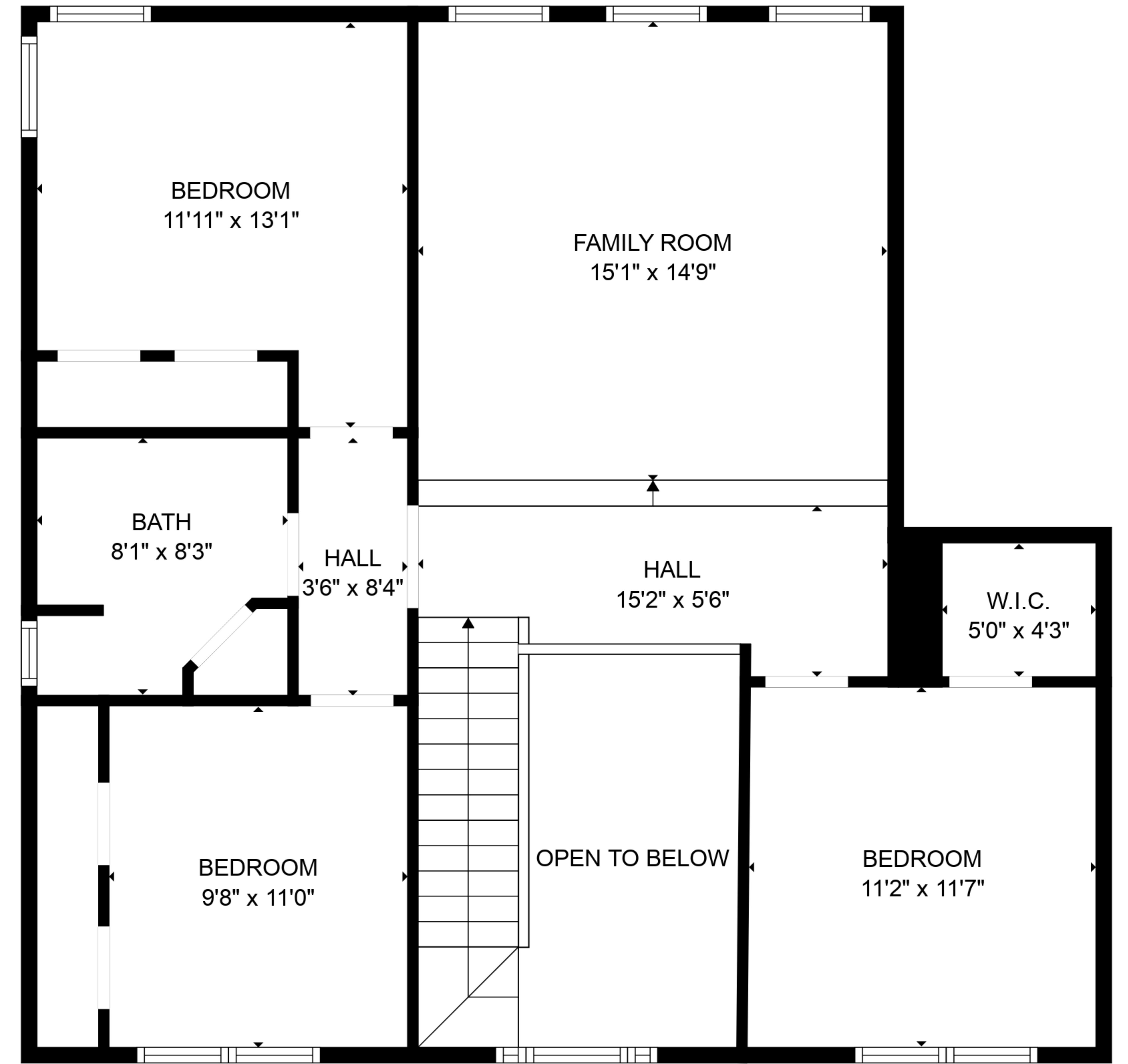
FLOOR 2
