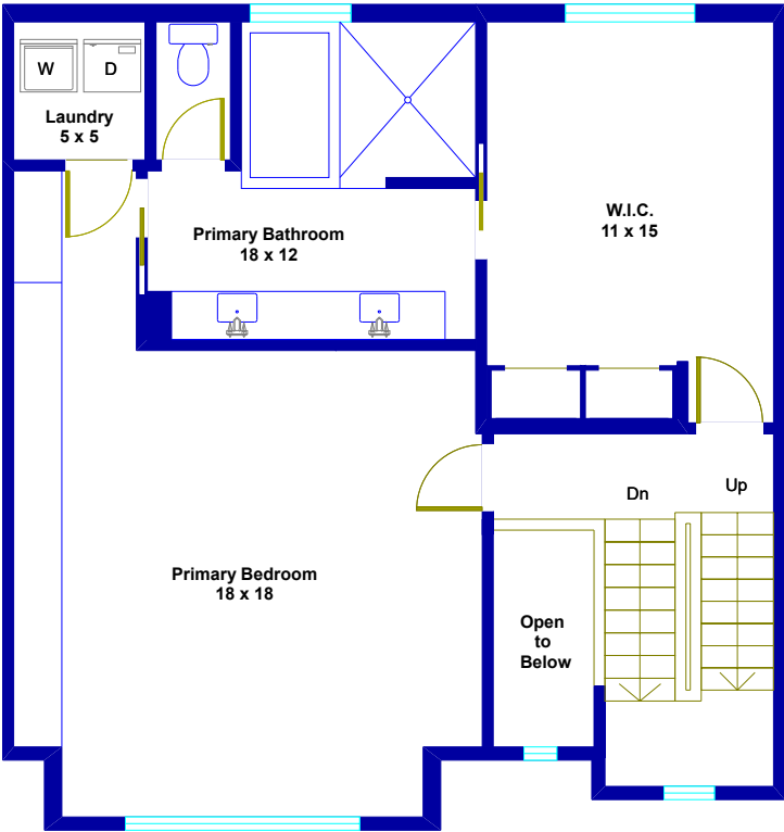
House Third Floor
