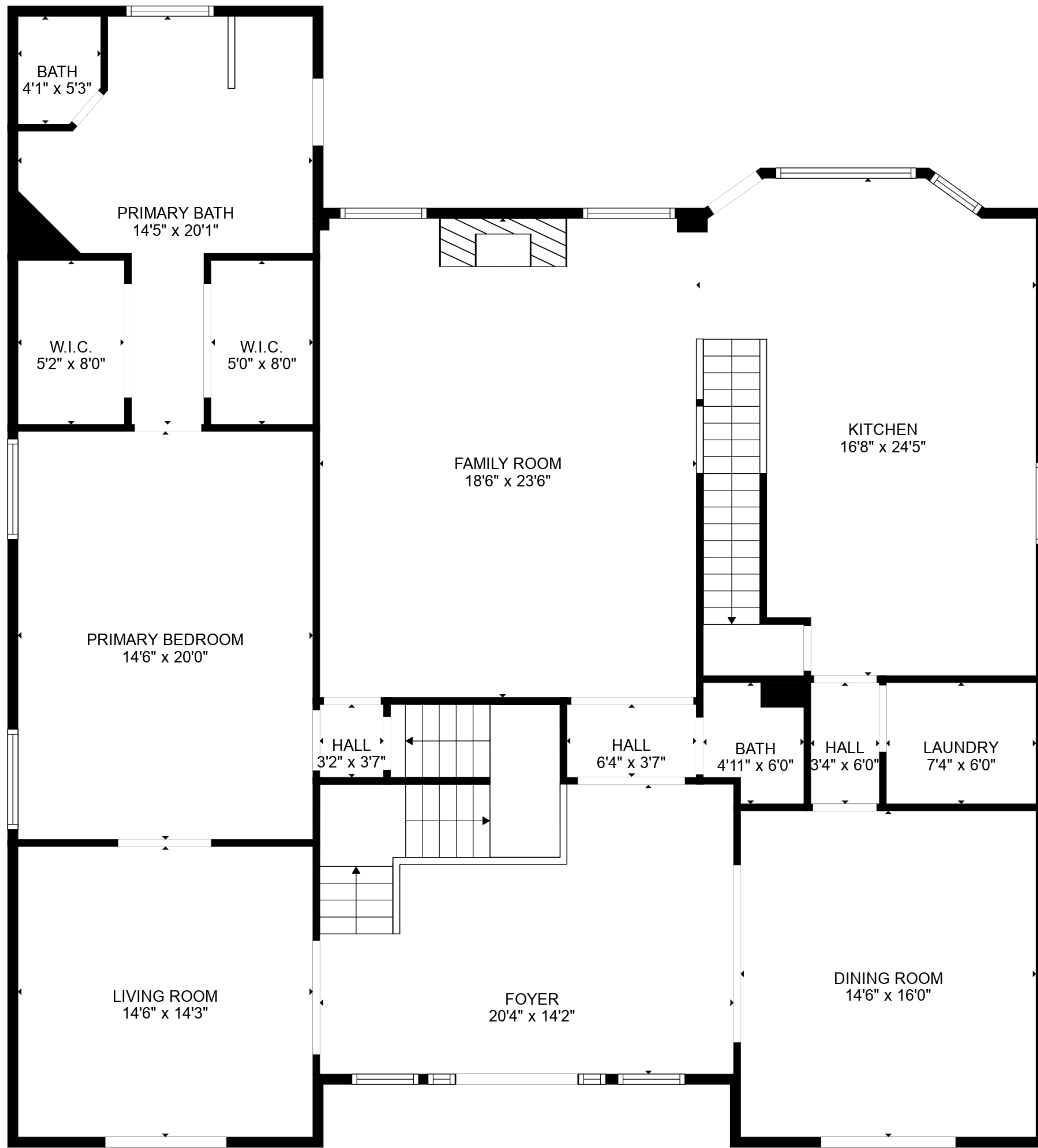
FLOOR 1
