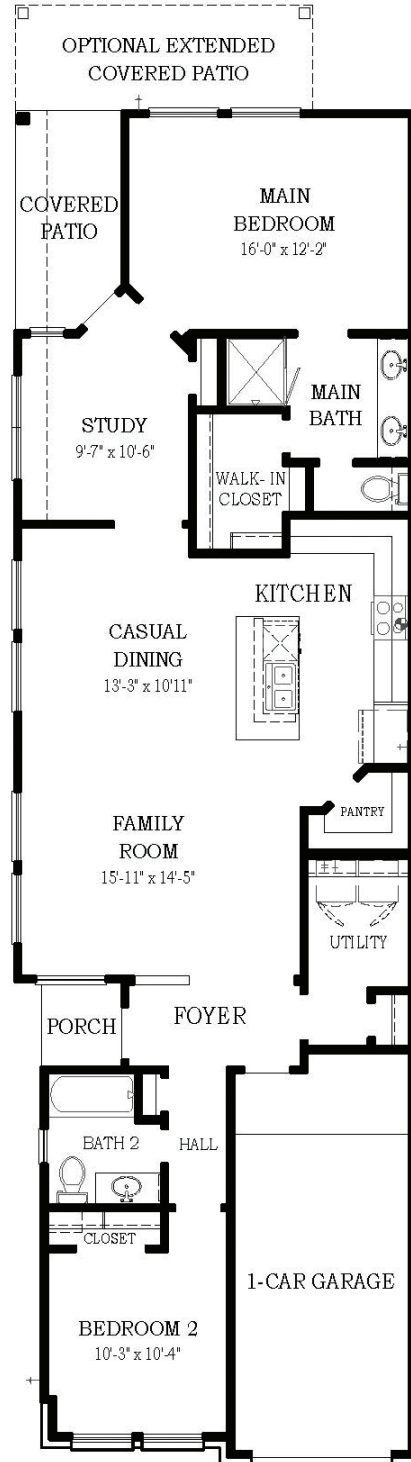
FLOOR PLAN
