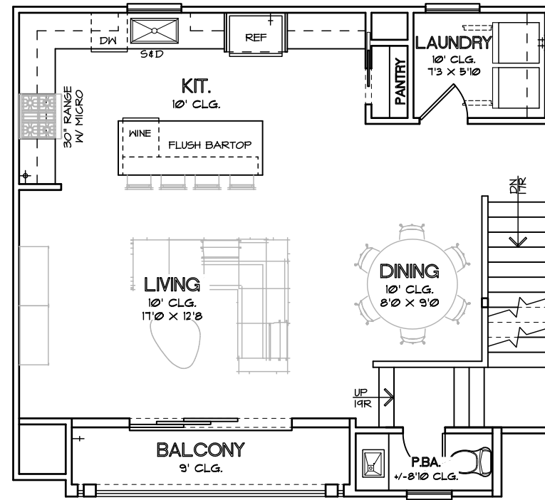
SECOND FLOOR PLAN PLAN 1788 R
