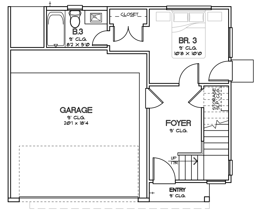
FIRST FLOOR PLAN PLAN 1788 R
