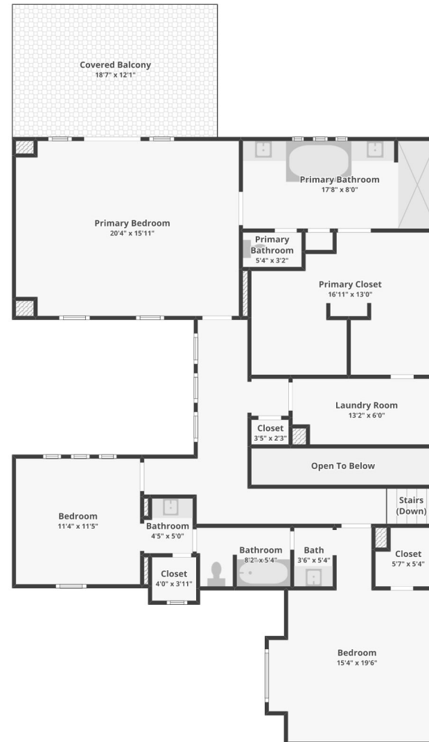
FLOOR 2
