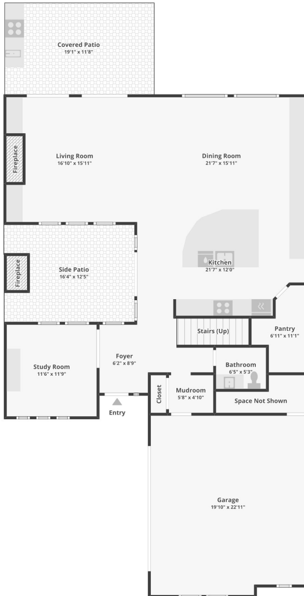
FLOOR 1
