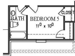
OPT. BEDROOM 5 WITH BATH 4 ( PLAN OPTION VARIES PER ELEVATION )
