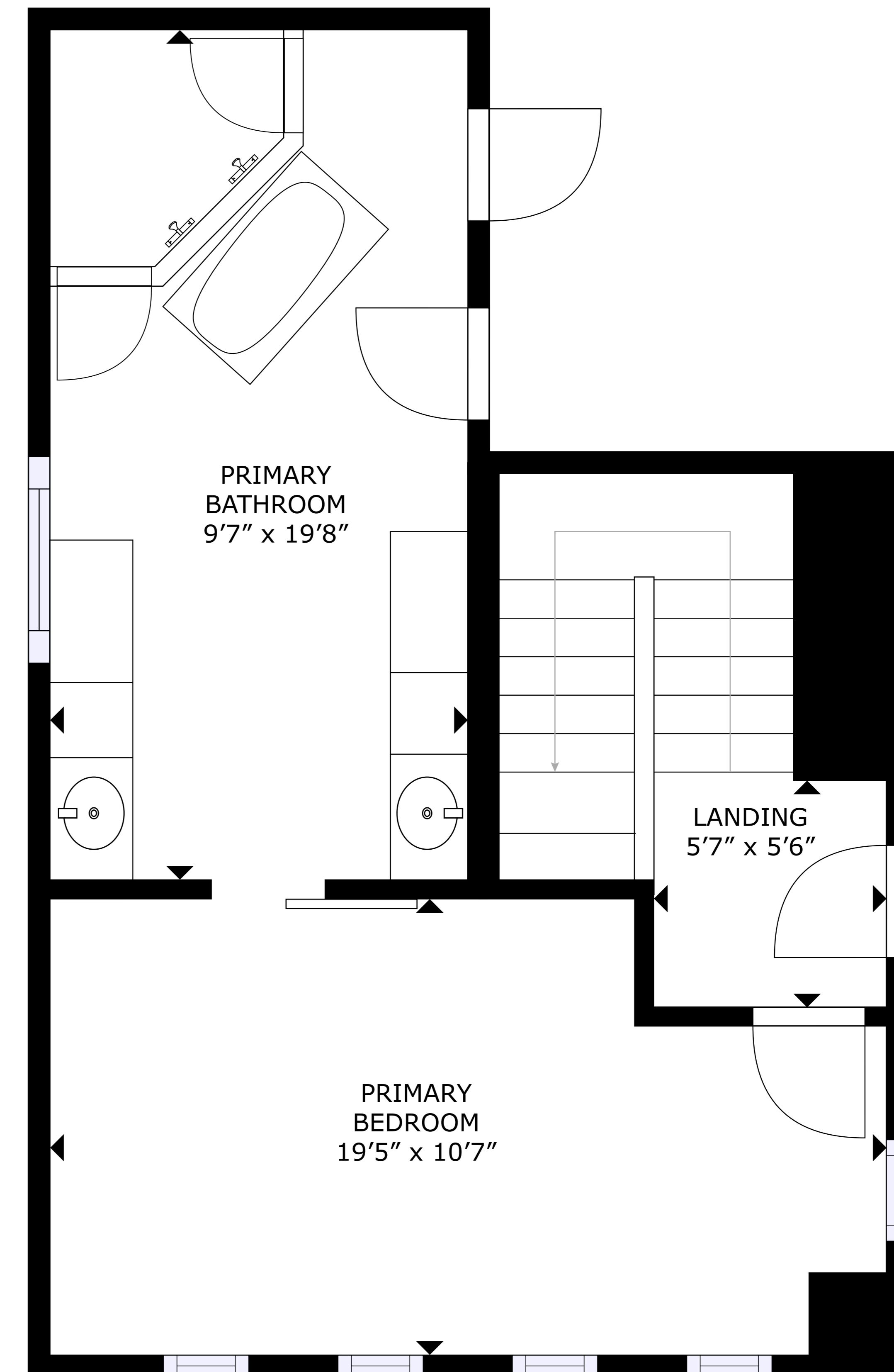
FLOOR 2
