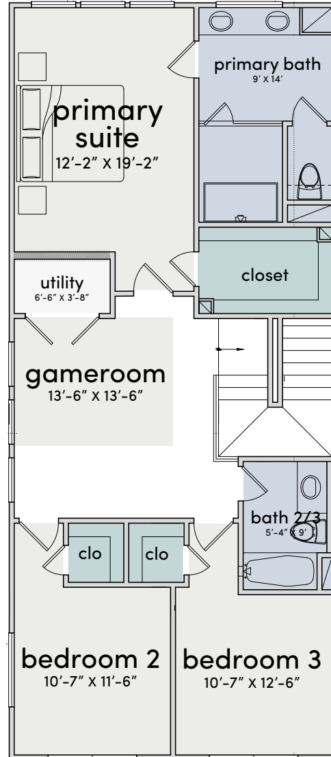
SECOND FLOOR
