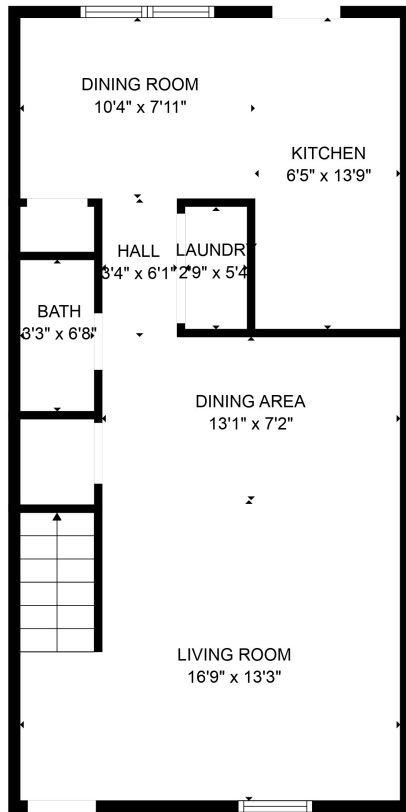
FLOOR 1
