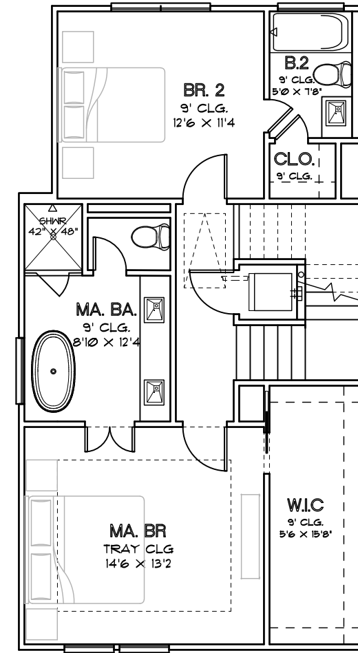
THIRD FLOOR PLAN PLAN 1859
