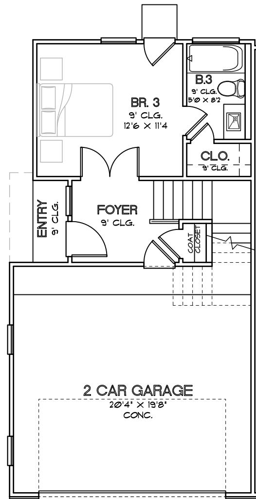
FIRST FLOOR PLAN PLAN 1859
