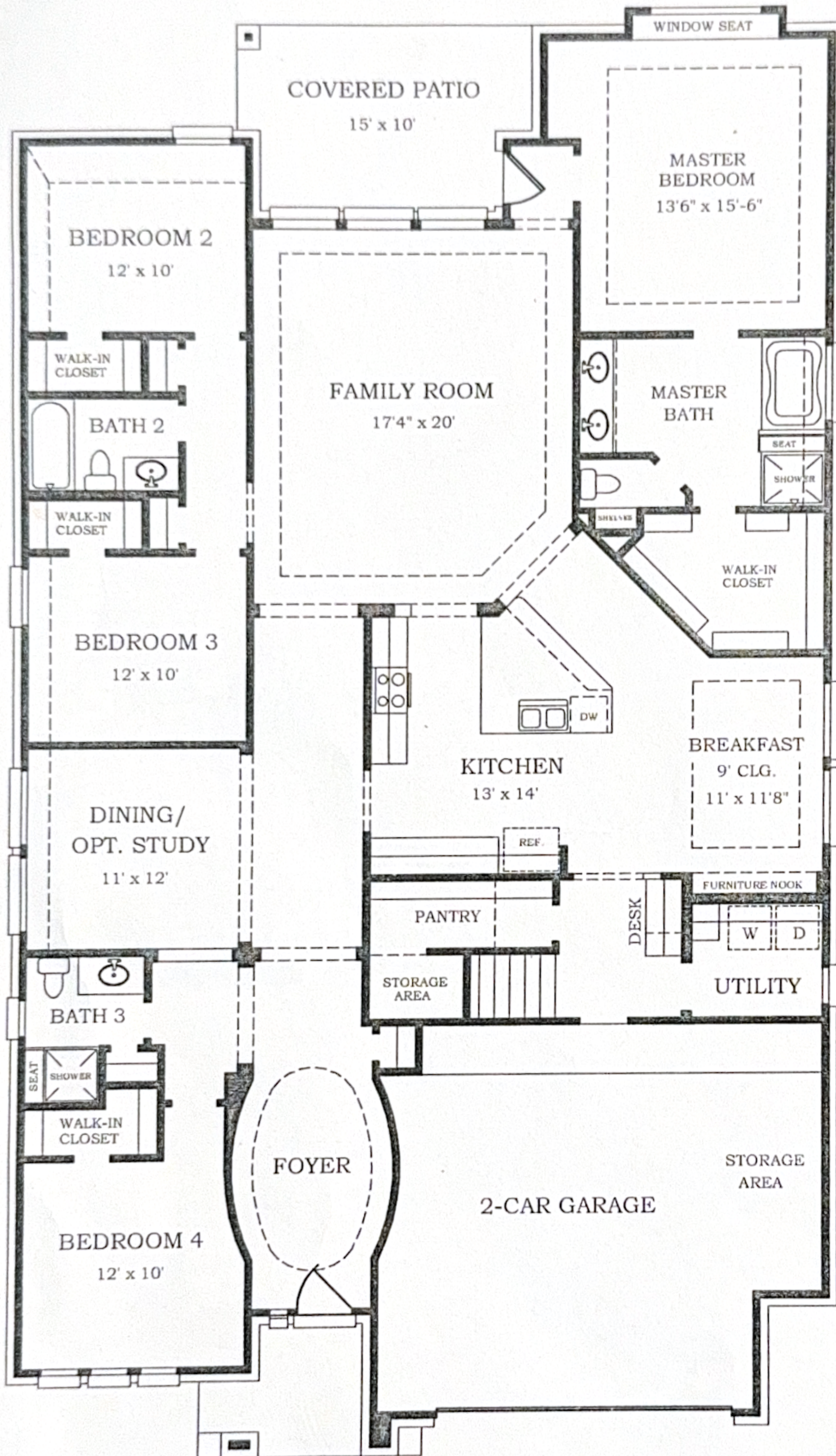
1st FLOOR
